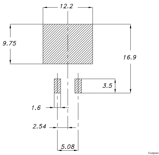
Figure 32. D 2 PAK (TO-263) recommended footprint (dimensions are in mm)
