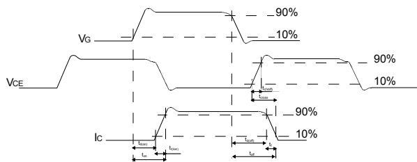
Figure 29. Switching waveform
