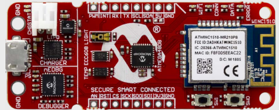
AVR-IoT WG Development Board (AC164160) PIC-IoT WG Development Board (AC164164)
