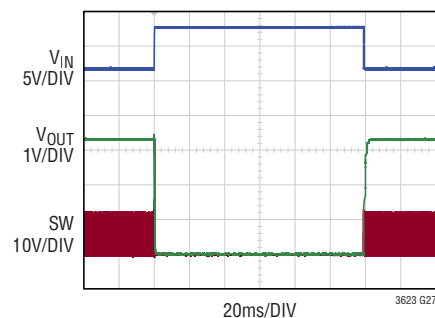
V_{IN} Overvoltage
