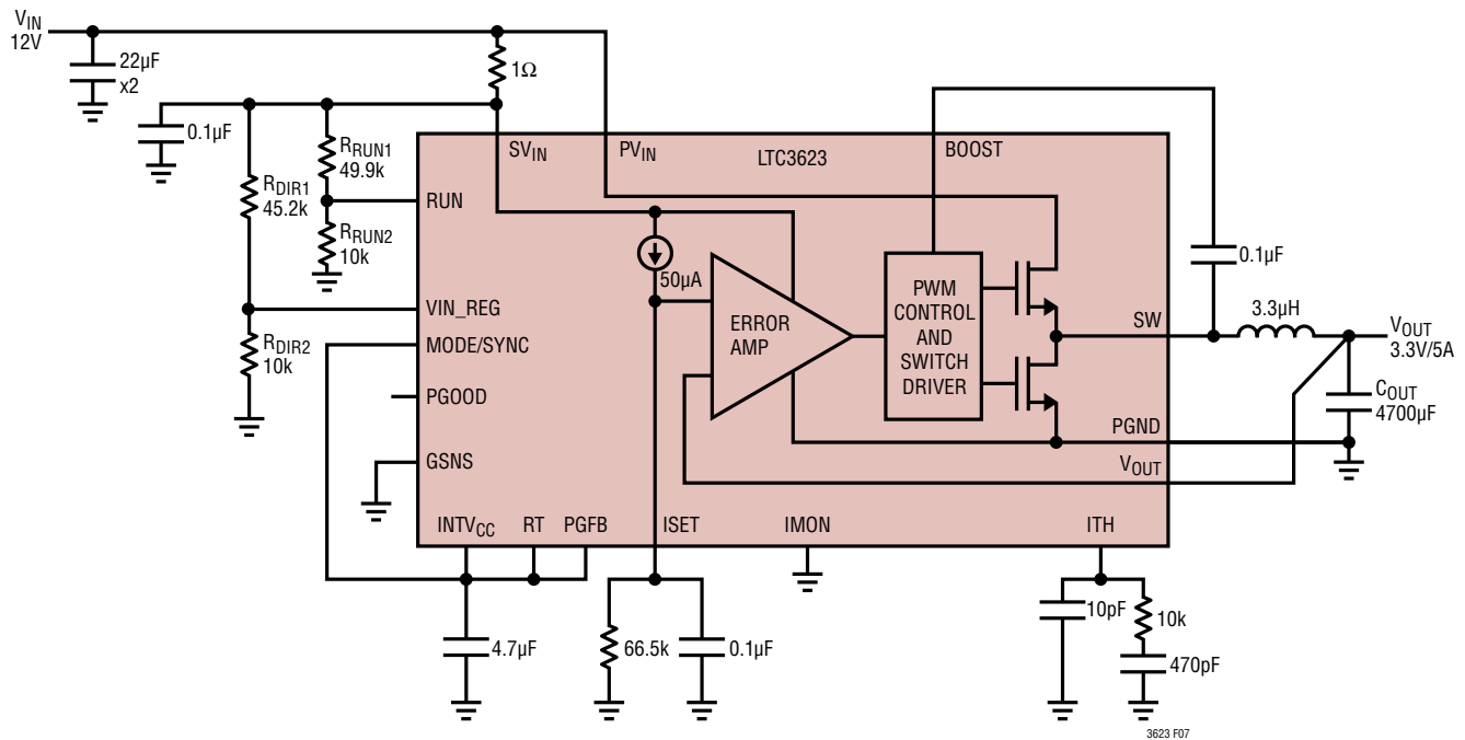
Figure 7. 12V to 3.3V 1MHz Buck Regulator with Input Supply Regulation Loop
