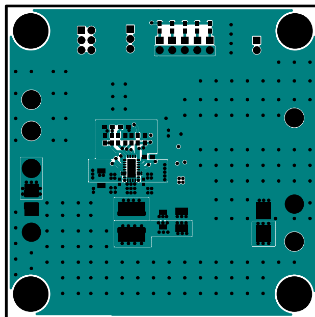
Figure 4. PCB Layout
