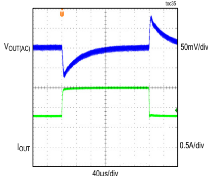
MAX17631A LOAD TRANSIENT BETWEEN 0.75A AND 1.5A FIGURE 3 CIRCUIT
