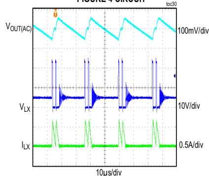
MAX17631B STEADY-STATE PERFORMANCE FIGURE 4 CIRCUIT
