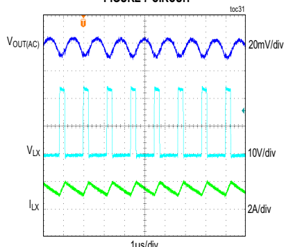
MAX17631C STEADY-STATE PERFORMANCE FIGURE 7 CIRCUIT
