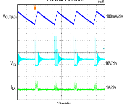
MAX17631C STEADY-STATE PERFORMANCE FIGURE 4 CIRCUIT
