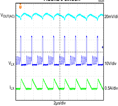
MAX17631A STEADY-STATE PERFORMANCE FIGURE 3 CIRCUIT
