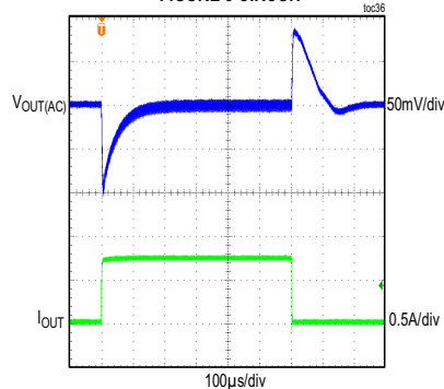
MAX17631A LOAD TRANSIENT BETWEEN 40mA AND 0.75A FIGURE 3 CIRCUIT
