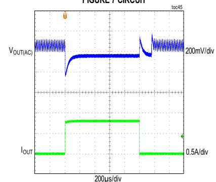
MAX17631C LOAD TRANSIENT BETWEEN 20mA AND 0.75A FIGURE 7 CIRCUIT
