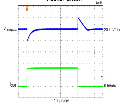
MAX17631C LOAD TRANSIENT BETWEEN 40mA AND 0.75A FIGURE 7 CIRCUIT
