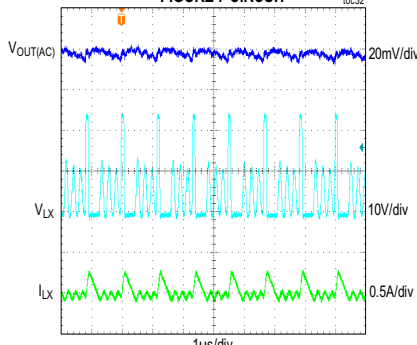
MAX17631C STEADY-STATE PERFORMANCE FIGURE 7 CIRCUIT
