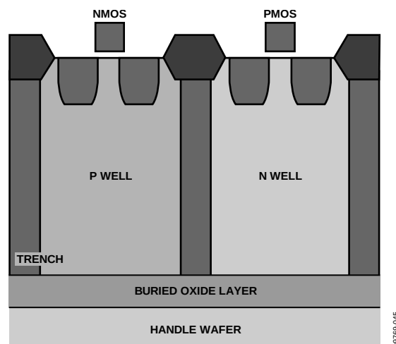
Figure 34. Trench Isolation
