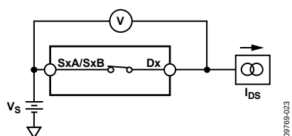
Figure 25. On Resistance
