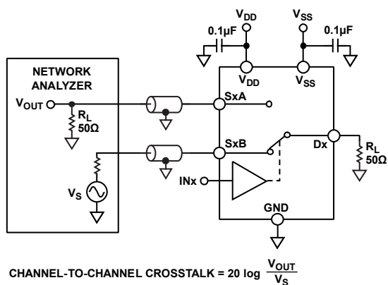
Figure 26. Channel-to-Channel Crosstalk
