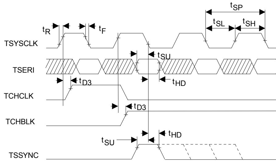
Figure 13-18. Transmit-Side Timing, Elastic Store Enabled
