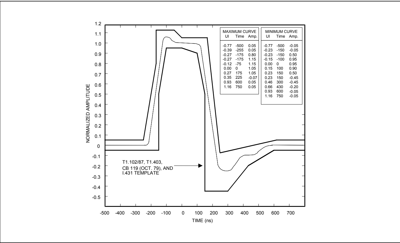
Figure 10-9. T1 Transmit Pulse Template
