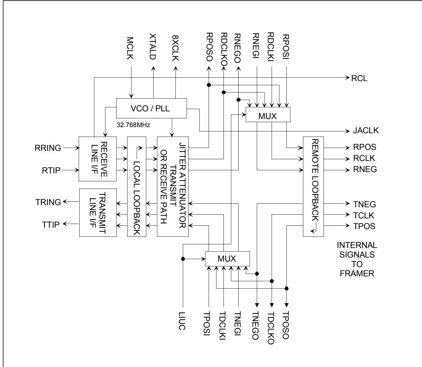
Figure 6-3. Receive and Transmit T1/E1/J1 LIU
