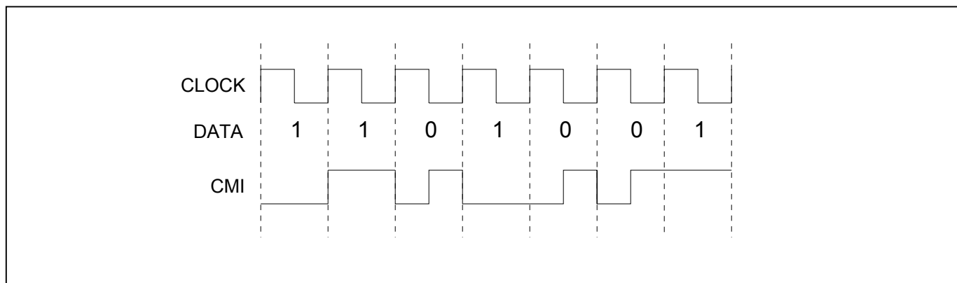
Figure 10-6. CMI Coding
