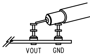
Figure 4. Measuring Output Ripple
