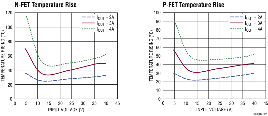
Figure 2. DC2234A Temperature Rising vs Input Voltage
