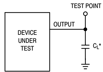
Figure 3. Test Circuit
