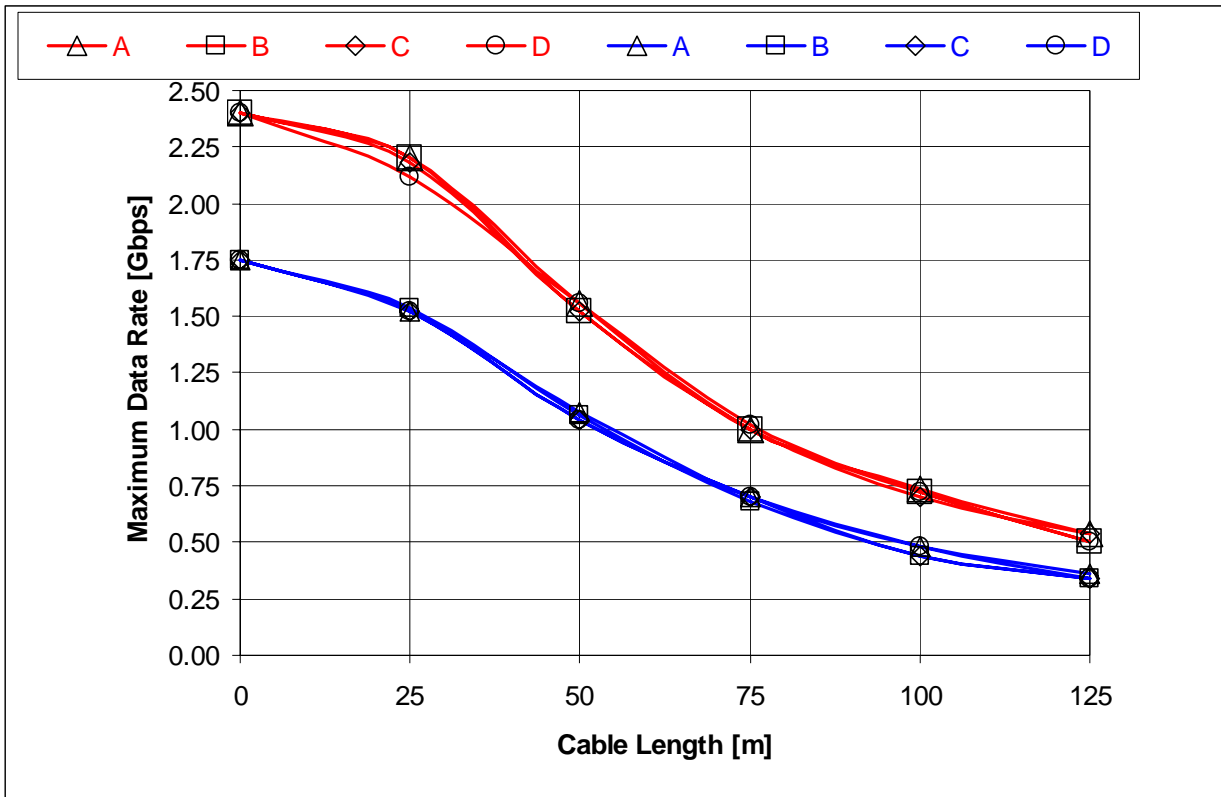
Figure 3. DS15BA101 and DS15EA101 Performance with CAT5e Cable
