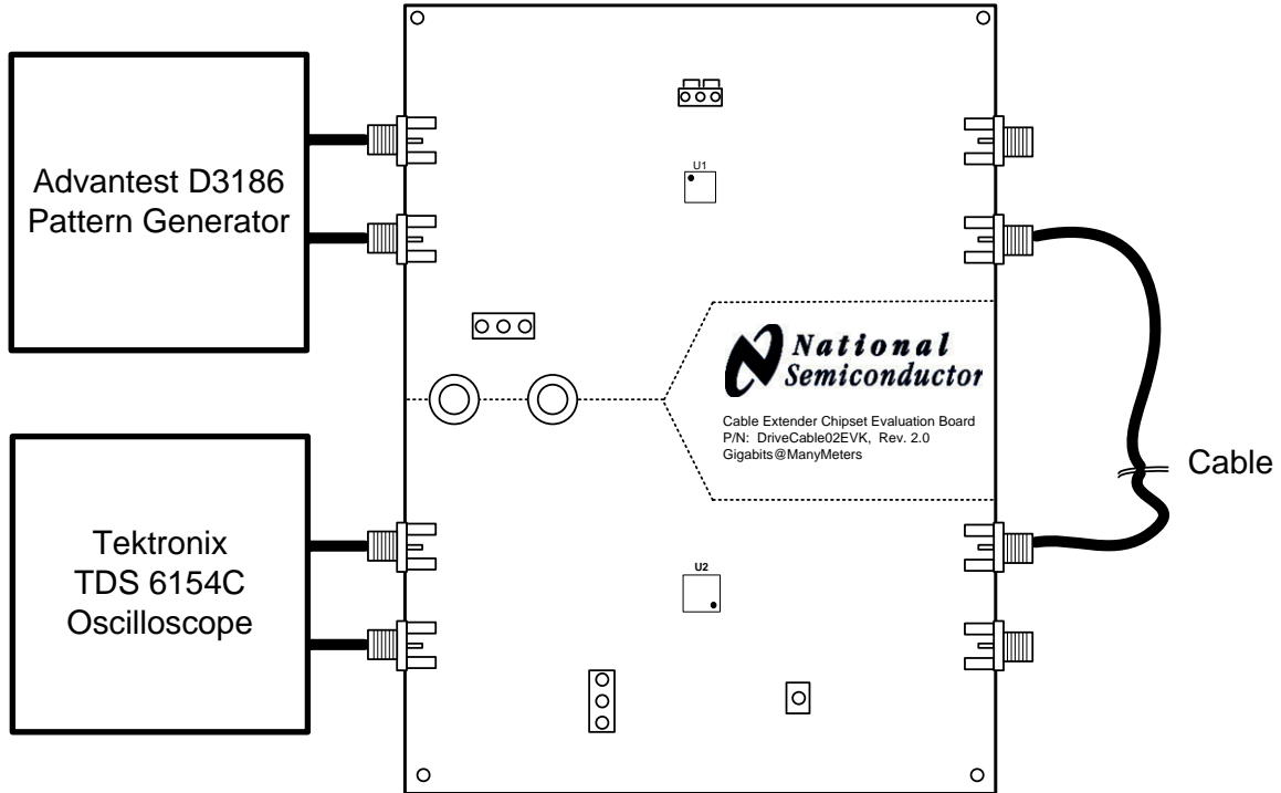
Figure 5. Test Setup for 50-ohm Coaxial Cable Evaluation
