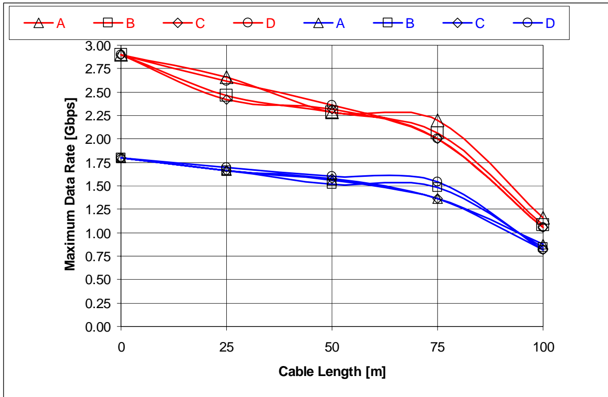
Figure 4. DS15BA101 and DS15EA101 Performance with CAT7 Cable
