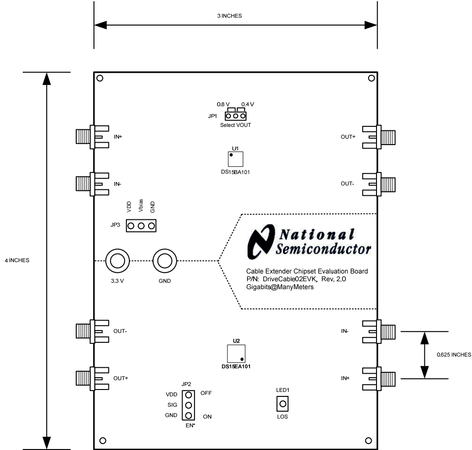
Figure 1. DriveCable02EVK Board
