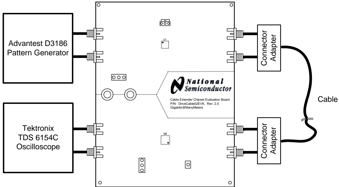
Figure 2. Test Setup for 100-ohm Differential Cable Evaluation
