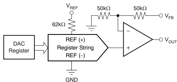
Figure 63. DAC8560 Architecture
