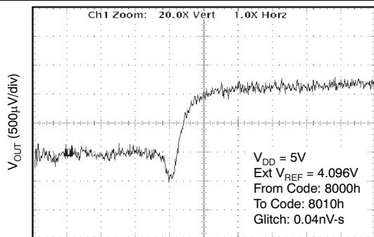
Figure 32. Glitch Energy
