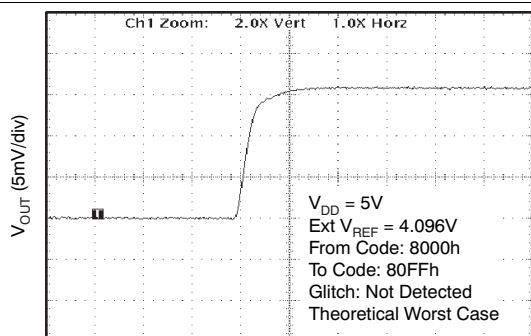
Figure 34. Glitch Energy
