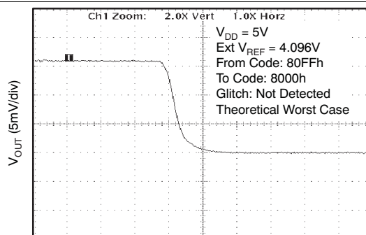
Figure 35. Glitch Energy
