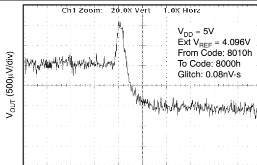
Figure 33. Glitch Energy
