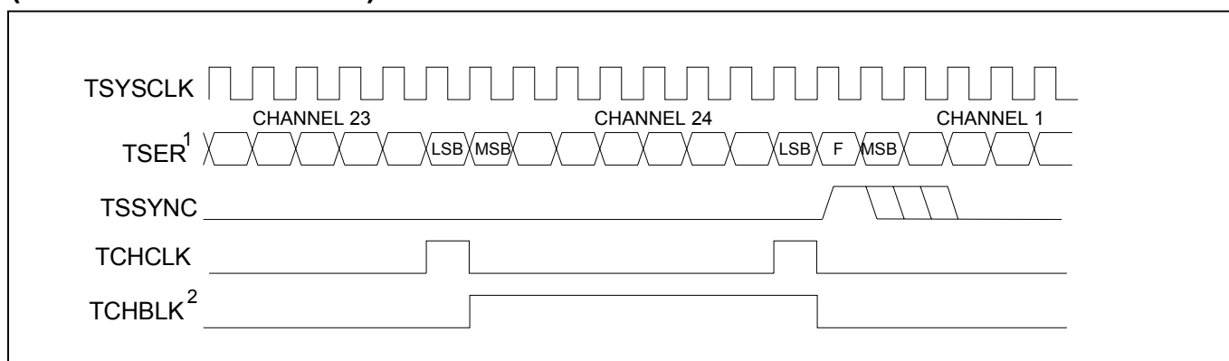
Figure 31-20. Transmit-Side Boundary Timing, TSYSClk = 1.544MHz (Elastic Store Enabled)
