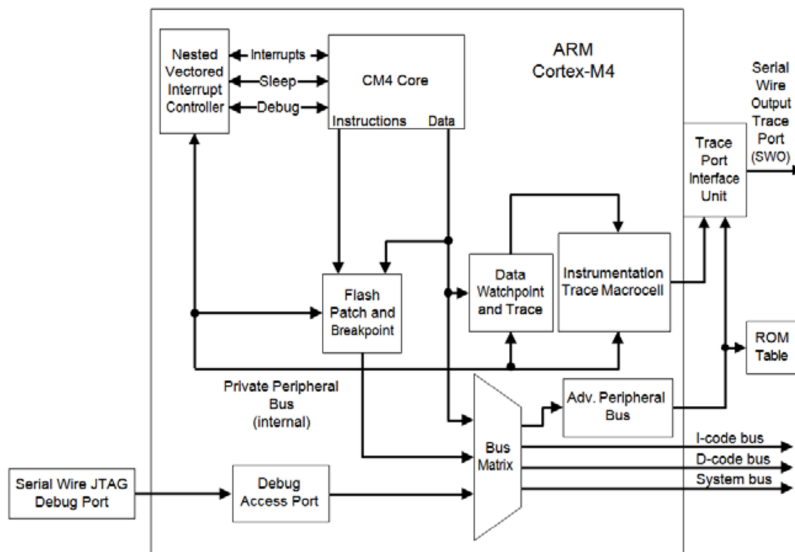
Figure 2-1. Application CPU Block Diagram
