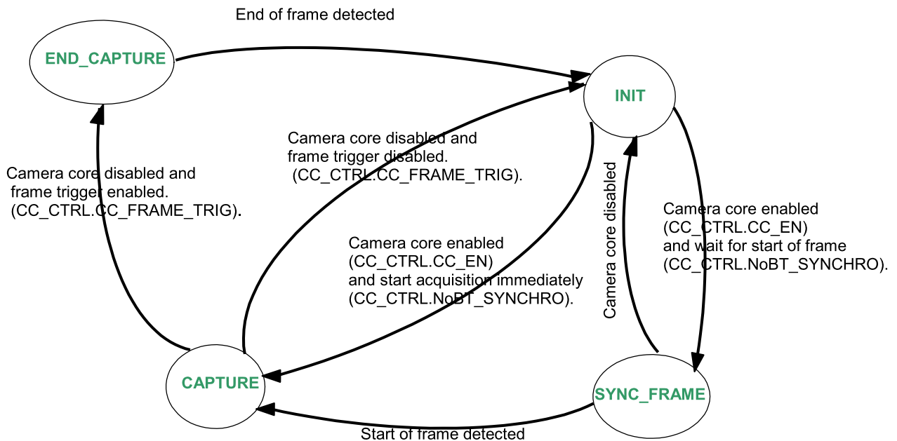
Figure 14-6. Parallel Camera I/F State Machine
