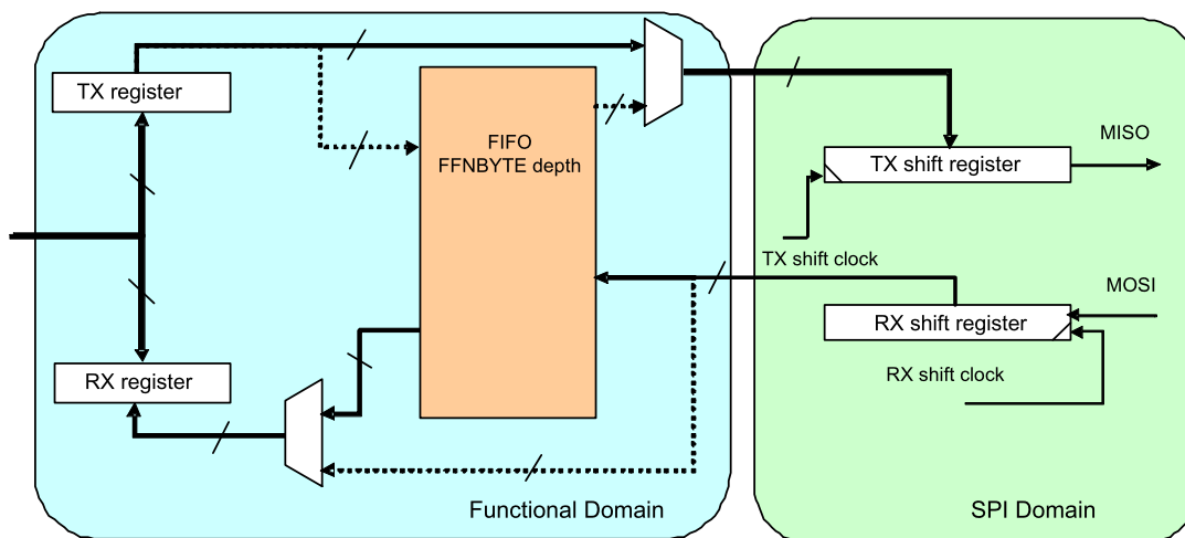
Figure 8-7. Transmit/Receive Mode With Only Receive FIFO Enabled
