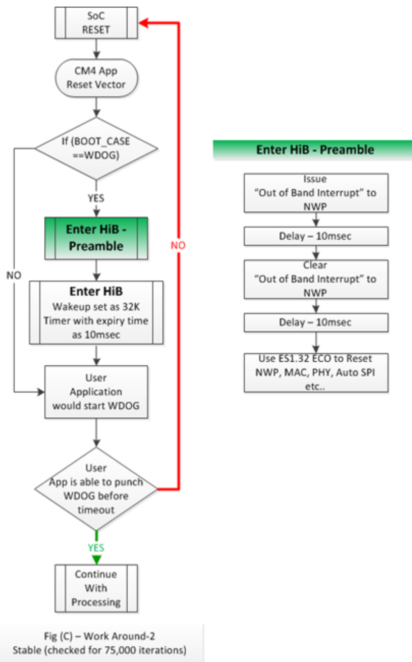
Figure 10-9. WatchDog Flow Chart
