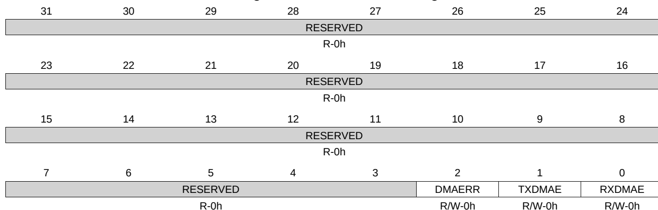
Figure 6-14. UARTDMACTL Register
