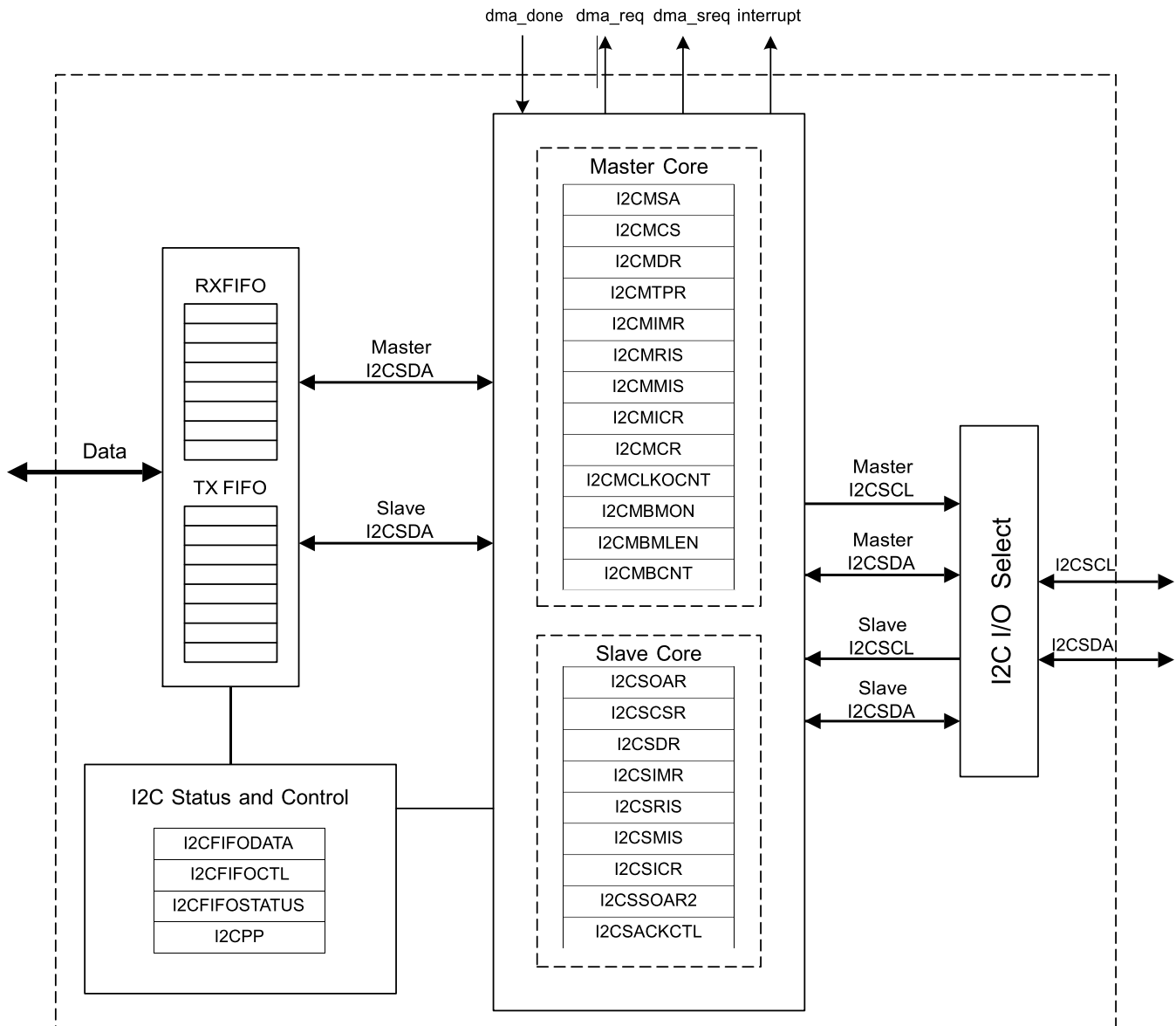
Figure 7-1. I2C Block Diagram
