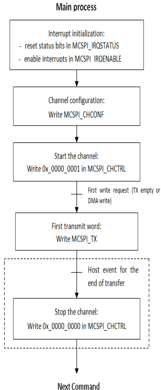
Figure 8-14. Flow Chart - Common Transfer Sequence
