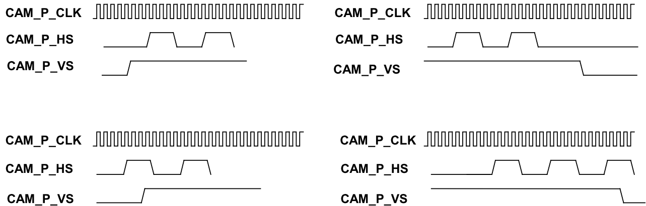
Figure 14-4. Different Scenarios of CAM_P_HS and CAM_P_VS Data is valid when both CAM_P_HS and CAM_P_VS are active (high in this example)
