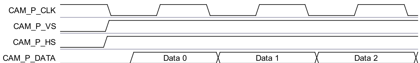
Figure 14-3. Synchronization Signals and Data Timing
