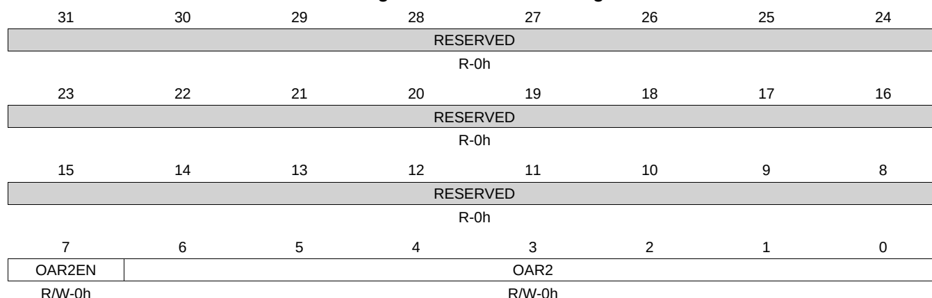
Figure 7-34. I2CSOAR2 Register
