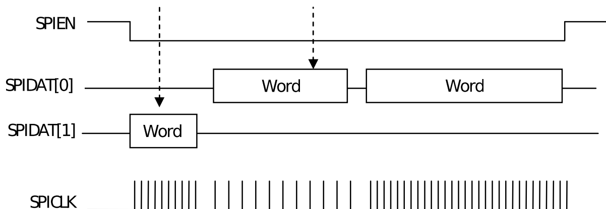
Figure 8-5. Contiguous Transfers with SPIEN Kept Active (2 Data Pins Interface Mode)
