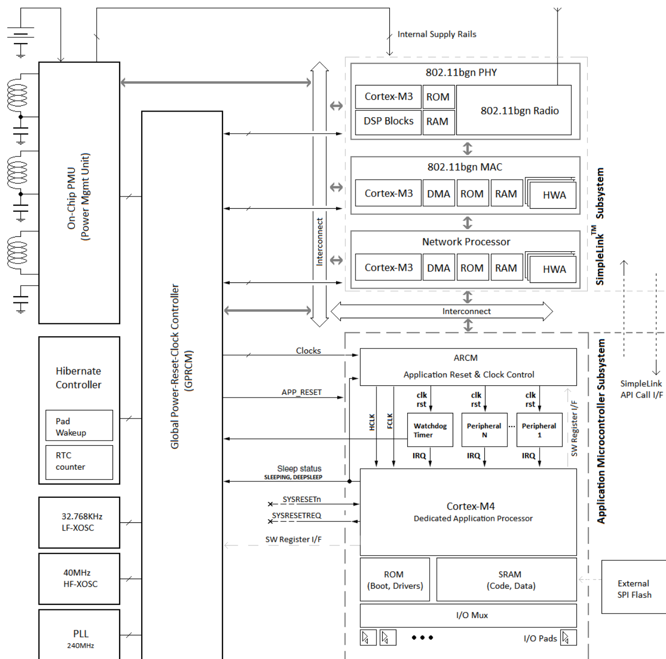
Figure 15-3. Power Management Control Architecture in CC3200
