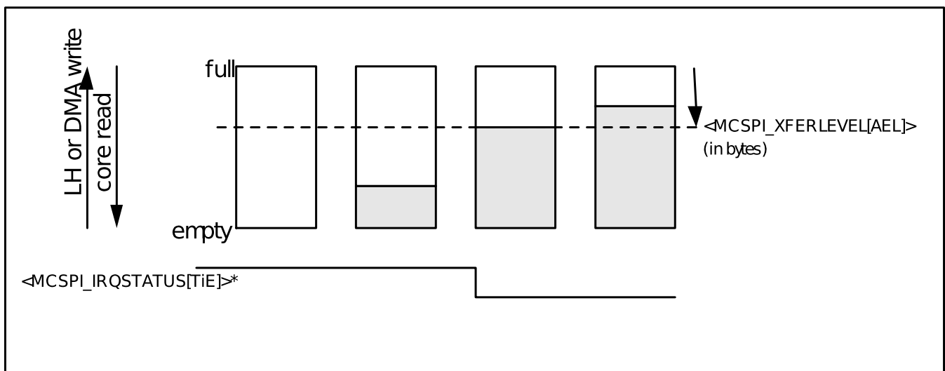
Figure 8-11. Buffer Almost Empty Level (AEL)
