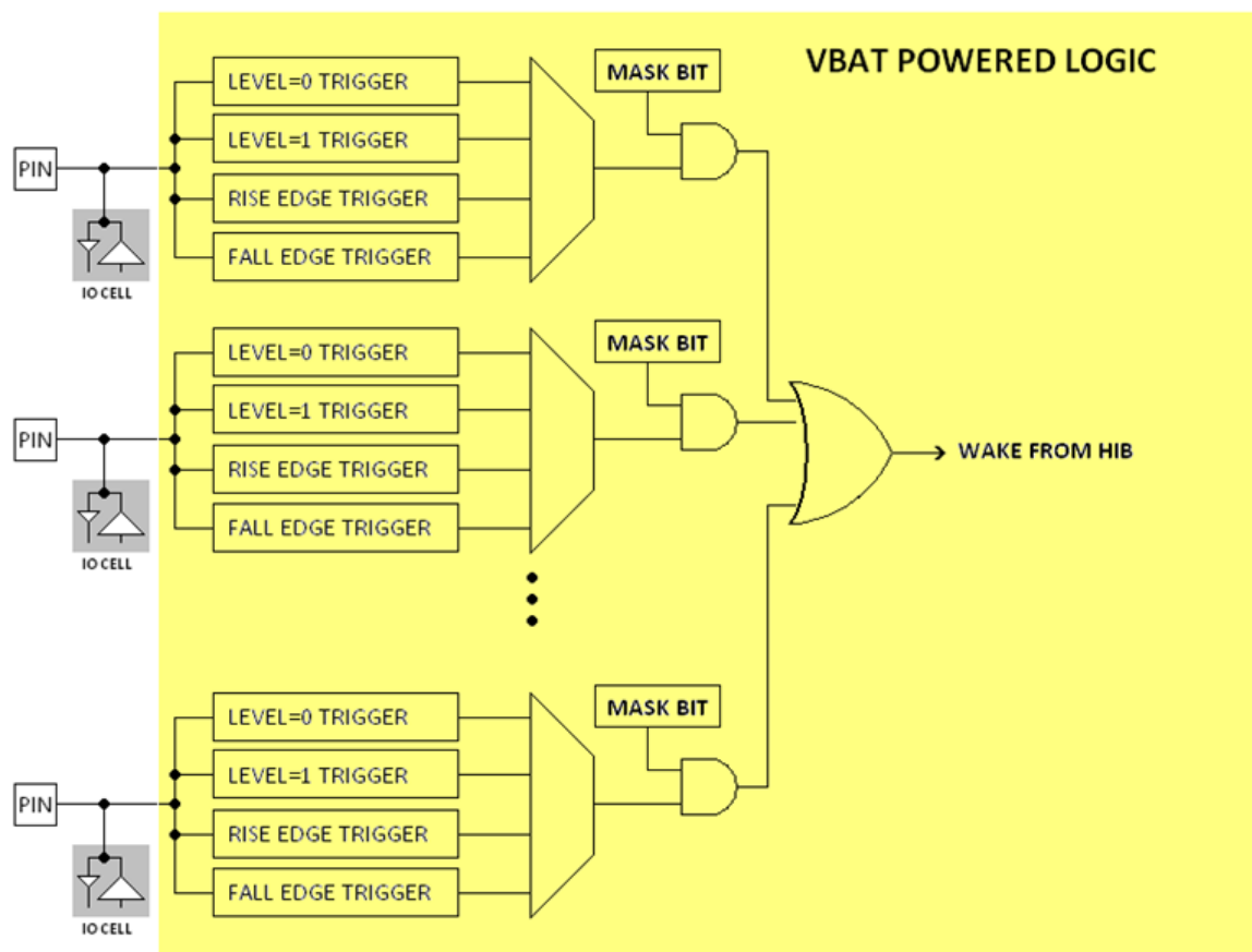
Figure 16-4. Wake on Pad for Hibernate Mode
