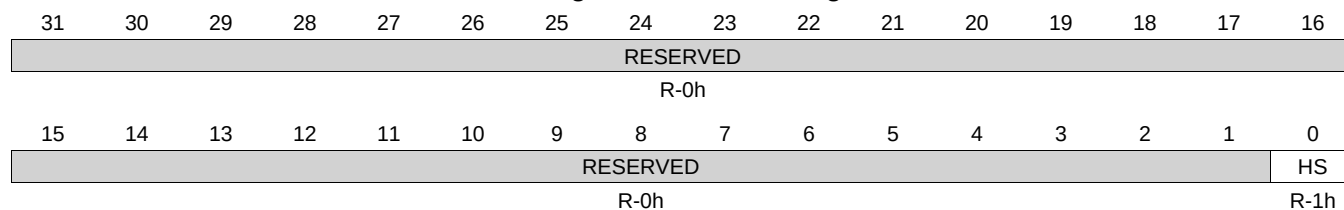
Figure 7-40. I2CPC Register
