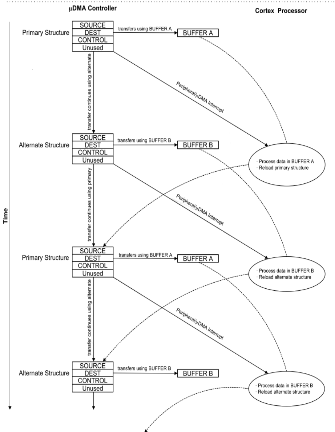
Figure 4-2. Ping-Pong Mode
