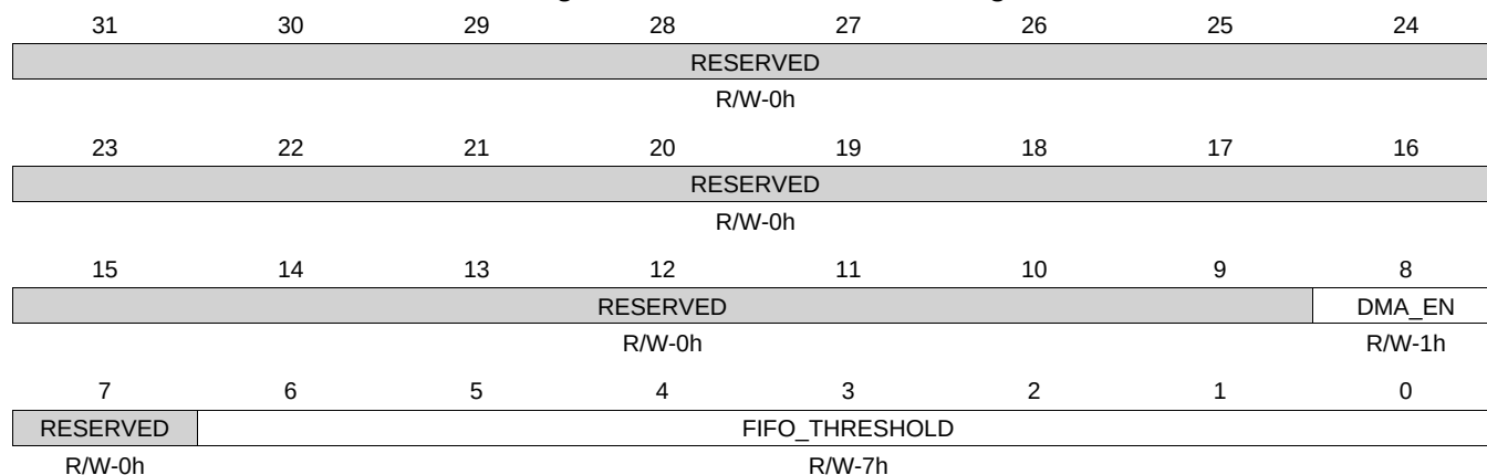
Figure 14-14. CC_CTRL_DMA Register
