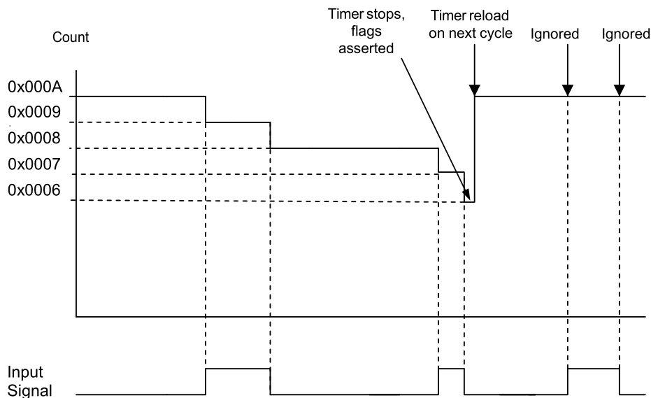
Figure 9-2. Input Edge-Count Mode Example, Counting Down
