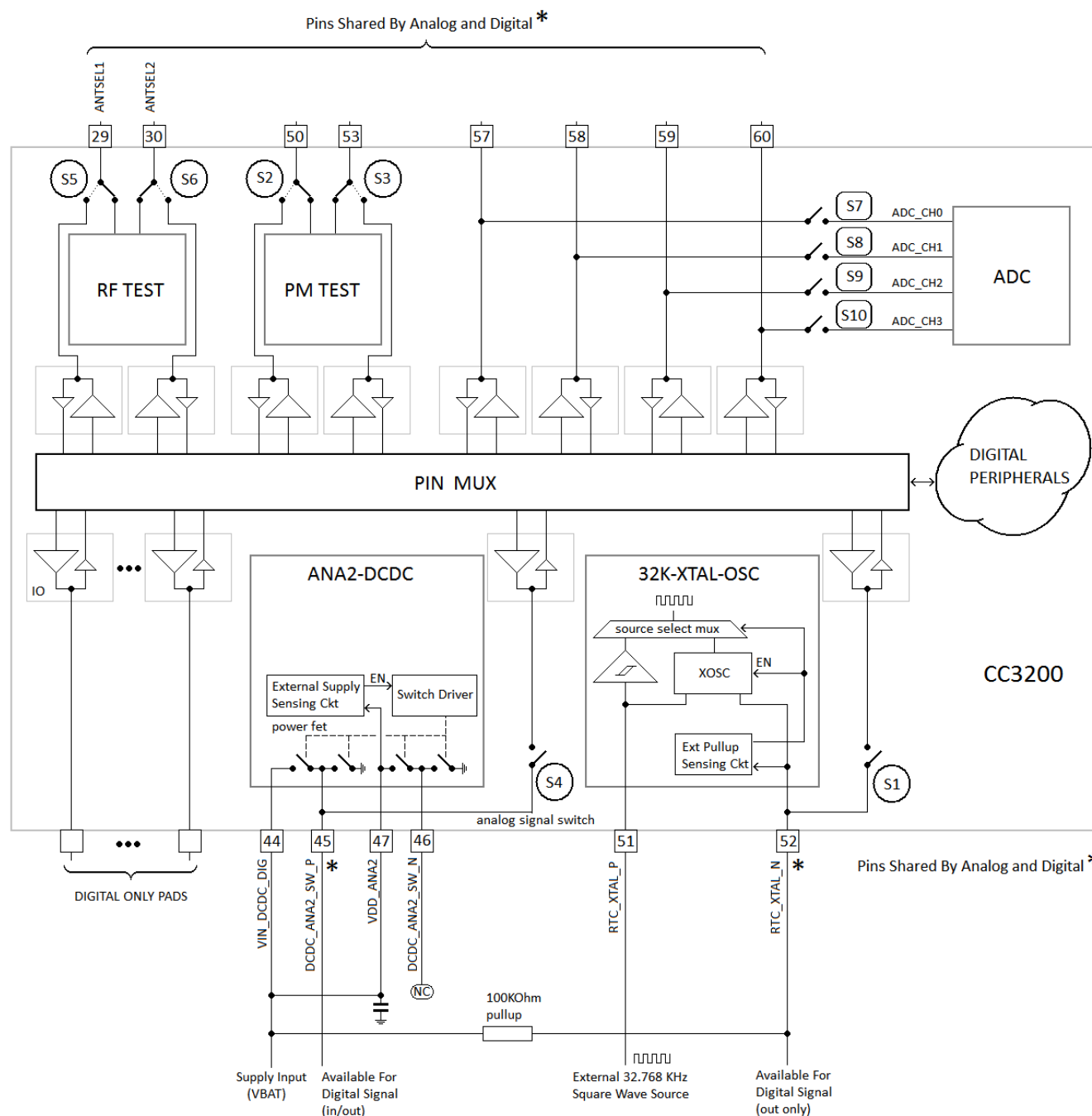
Figure 16-2. Board Configuration to Use Pins 45 and 52 as Digital Signals
