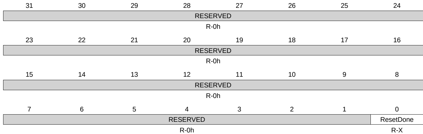
Figure 14-10. CC_SYSSTATUS Register
