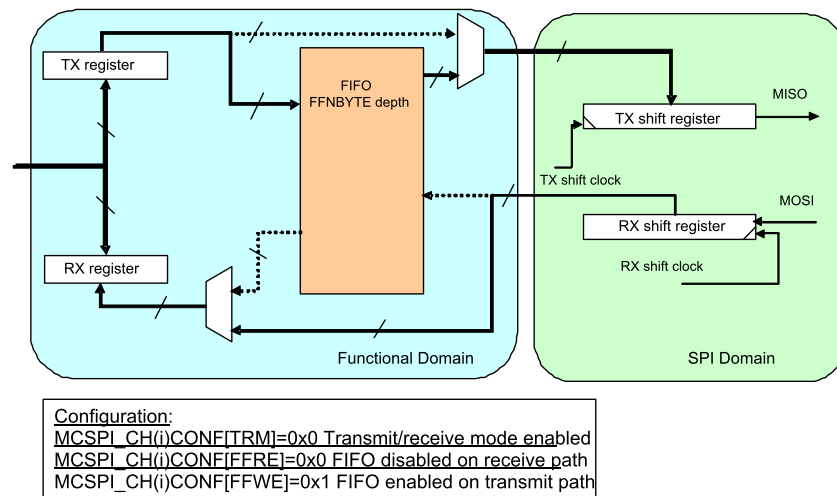
Figure 8-9. Transmit/Receive Mode With Both FIFO Directions Used
