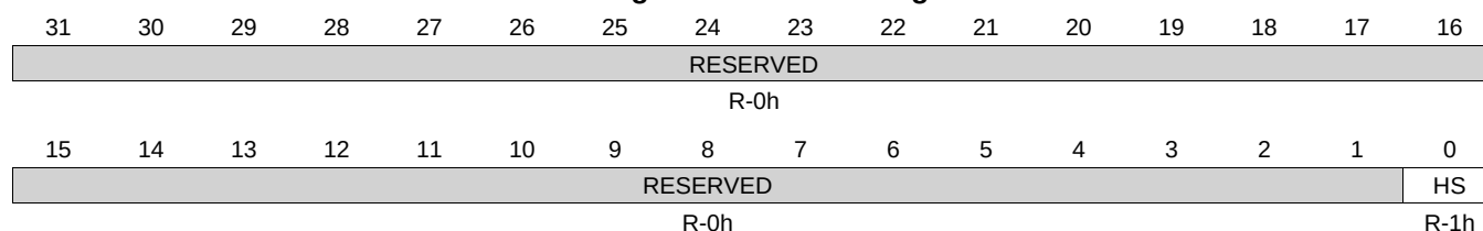
Figure 7-39. I2CPP Register
