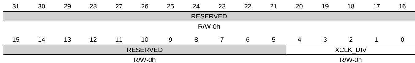
Figure 14-15. CC_CTRL_XCLK Register
