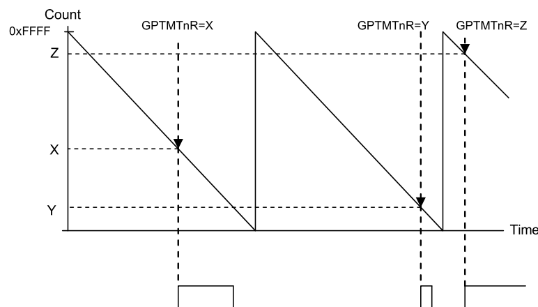
Figure 9-3. 16-Bit Input Edge-Time Mode Example
