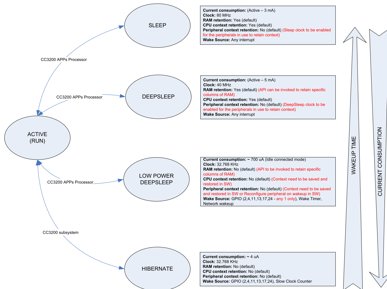
Figure 15-2. Sleep Modes
