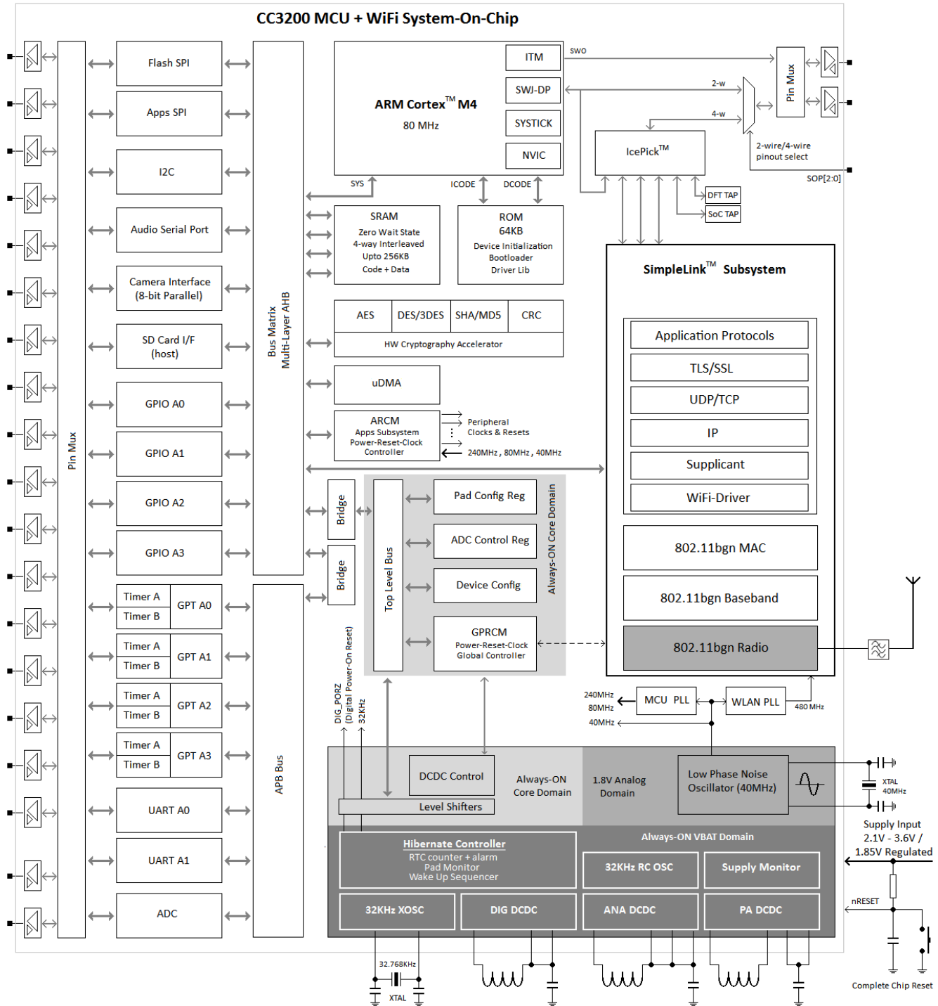
Figure 1-1. CC3200 MCU and WiFi System-on-Chip
