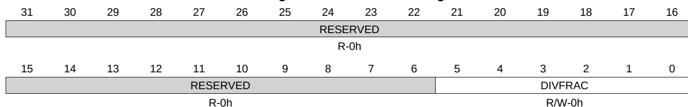
Figure 6-6. UARTFBRD Register
