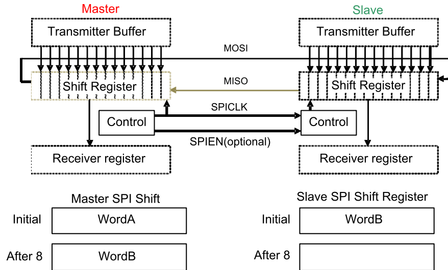
Figure 8-2. SPI Full Duplex Transmission (Example)
