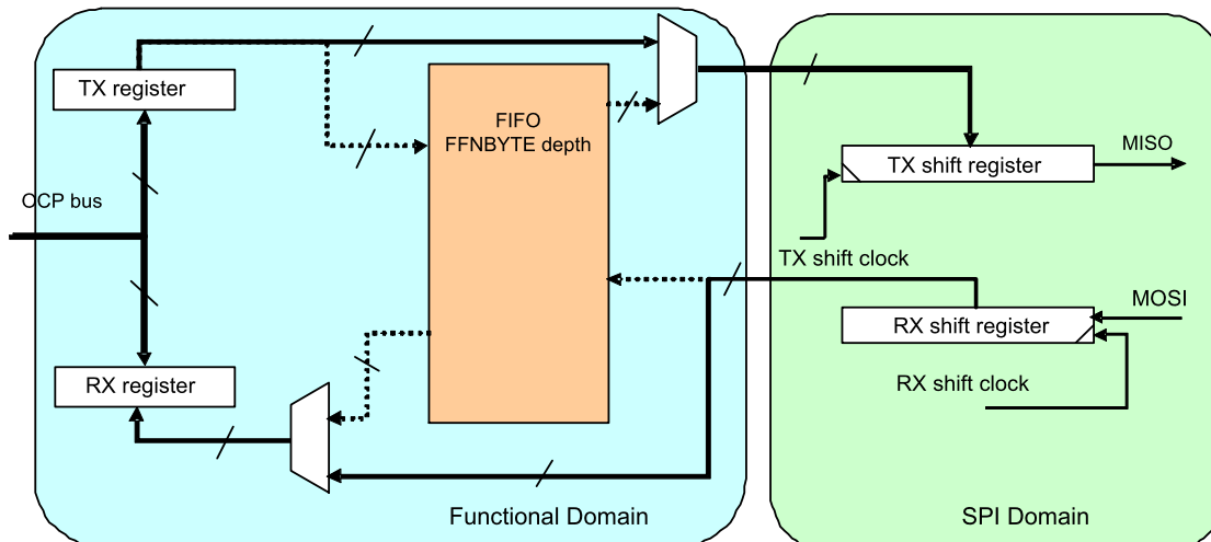
Figure 8-6. Transmit/Receive Mode With no FIFO Used
