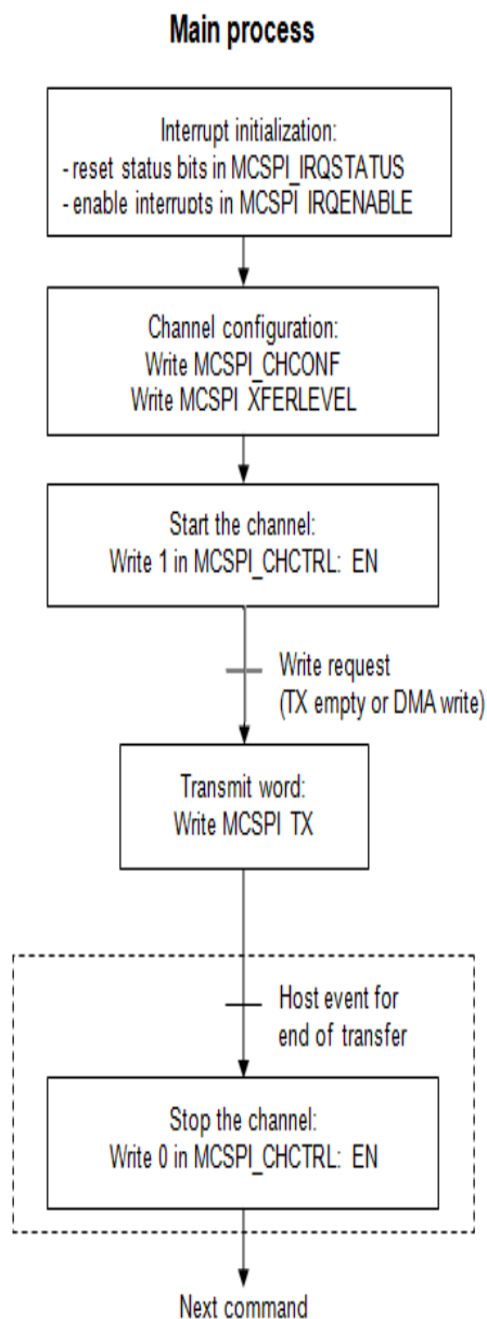
Figure 8-16. Flow Chart - FIFO Mode Common Sequence (Master)
