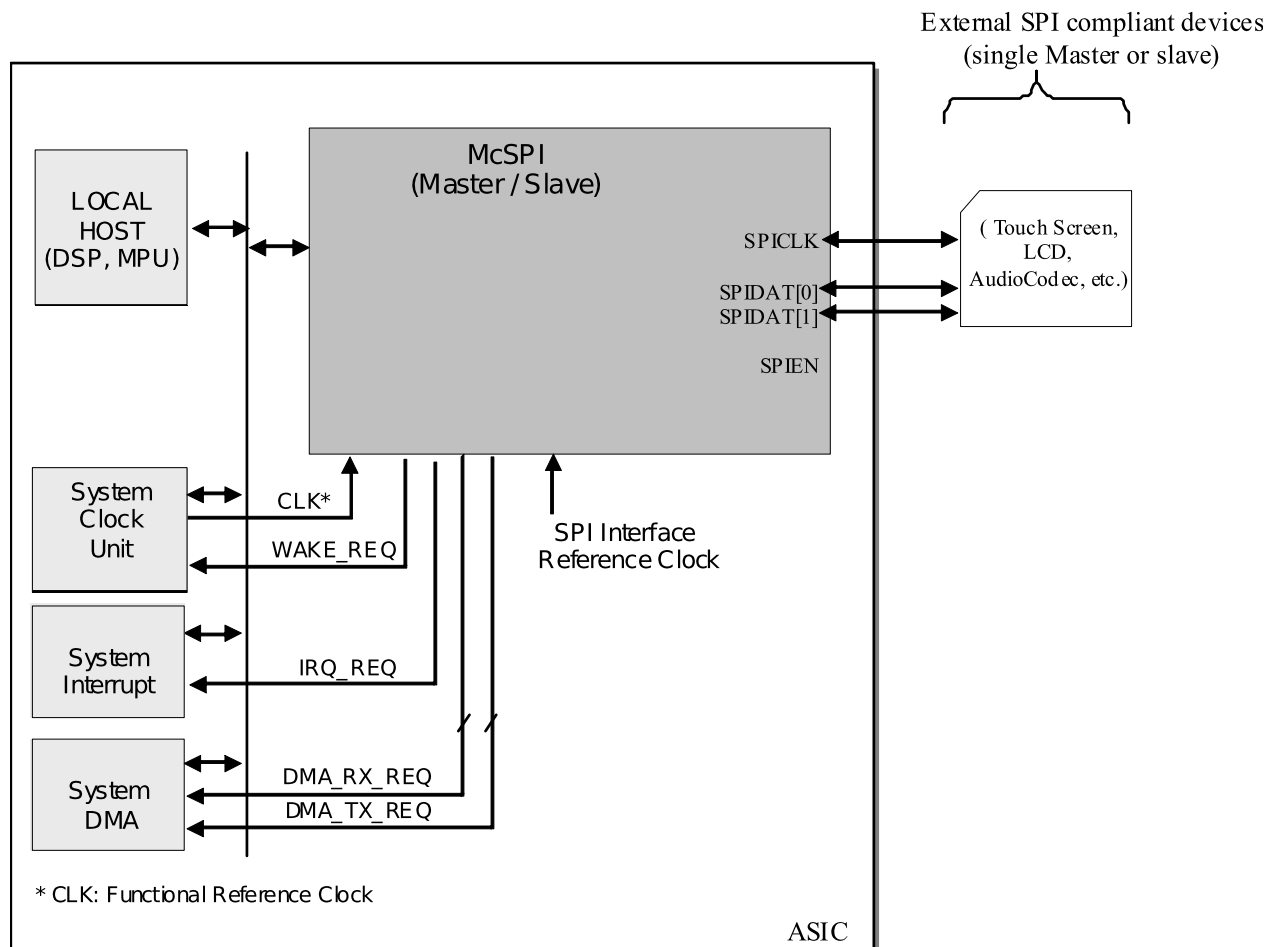
Figure 8-12. 3-Pin Mode System Overview
