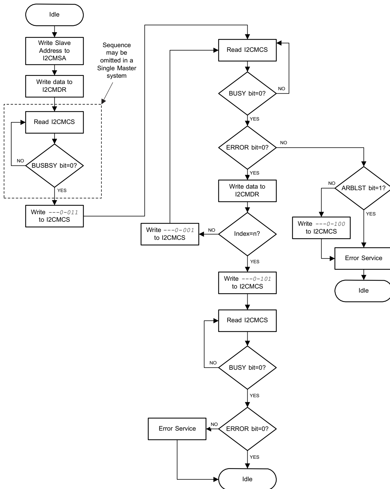
Figure 7-9. Master TRANSMIT of Multiple Data Bytes
