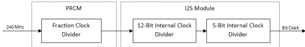
Figure 12-3. Logical Clock Path
