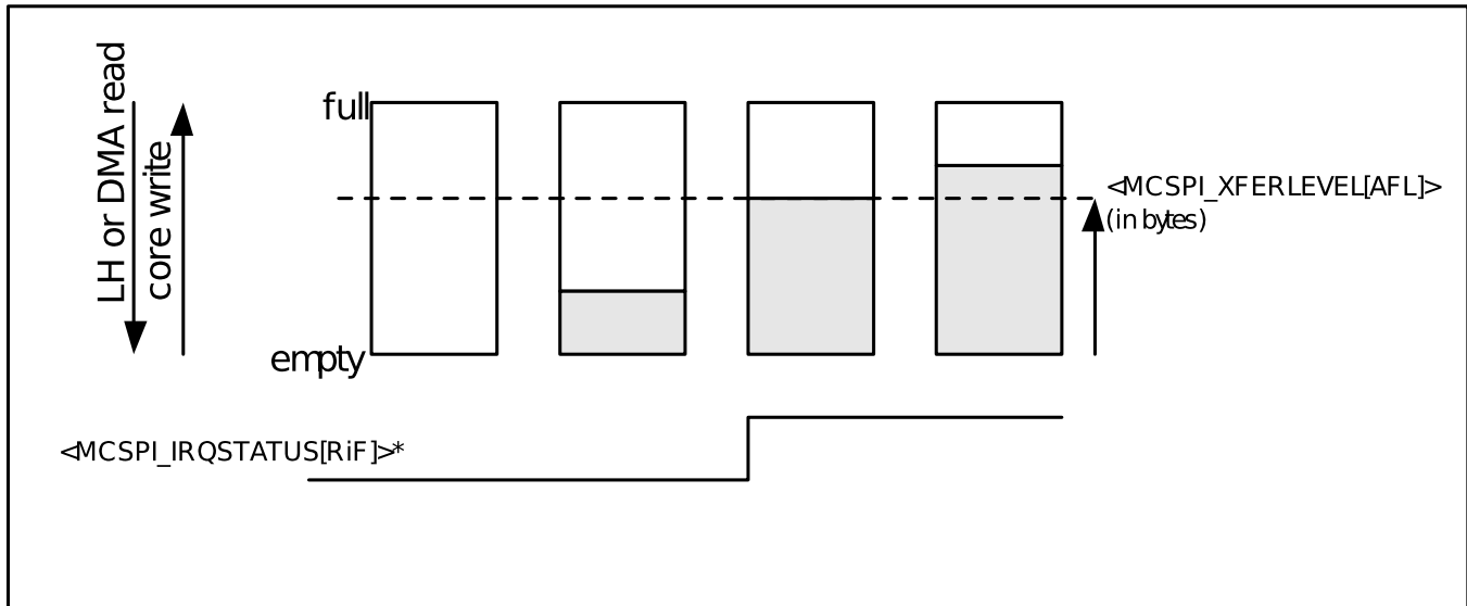
Figure 8-10. Buffer Almost Full Level (AFL)
