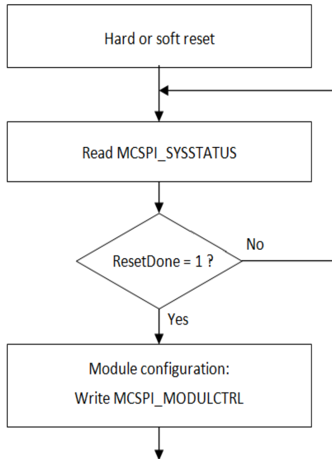
Figure 8-13. Flow Chart - Module Initialization
