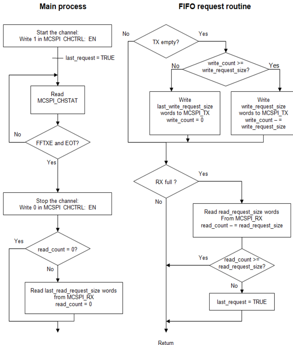
Figure 8-18. Flow Chart - FIFO Mode Transmit and Receive without Word Count (Master)
