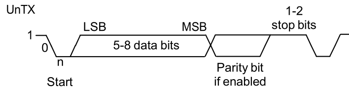
Figure 6-2. UART Character Frame
