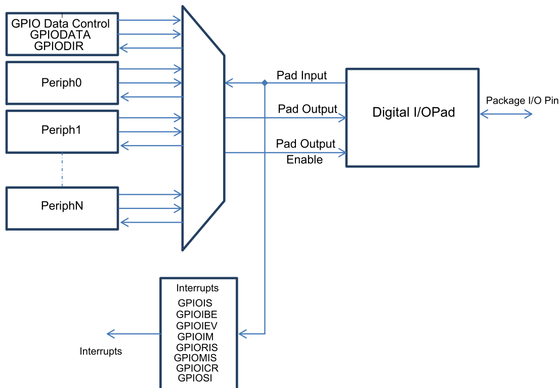
Figure 5-1. Digital I/O Pads
