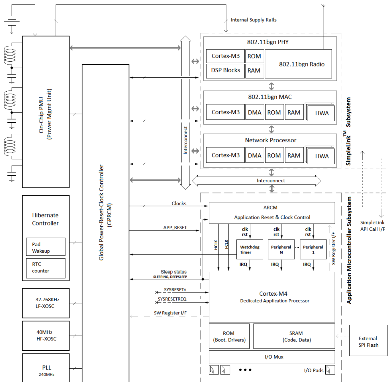
Figure 2-7. Power Management Architecture in CC3200 SoC
