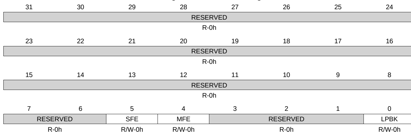
Figure 7-22. I2CMCR Register
