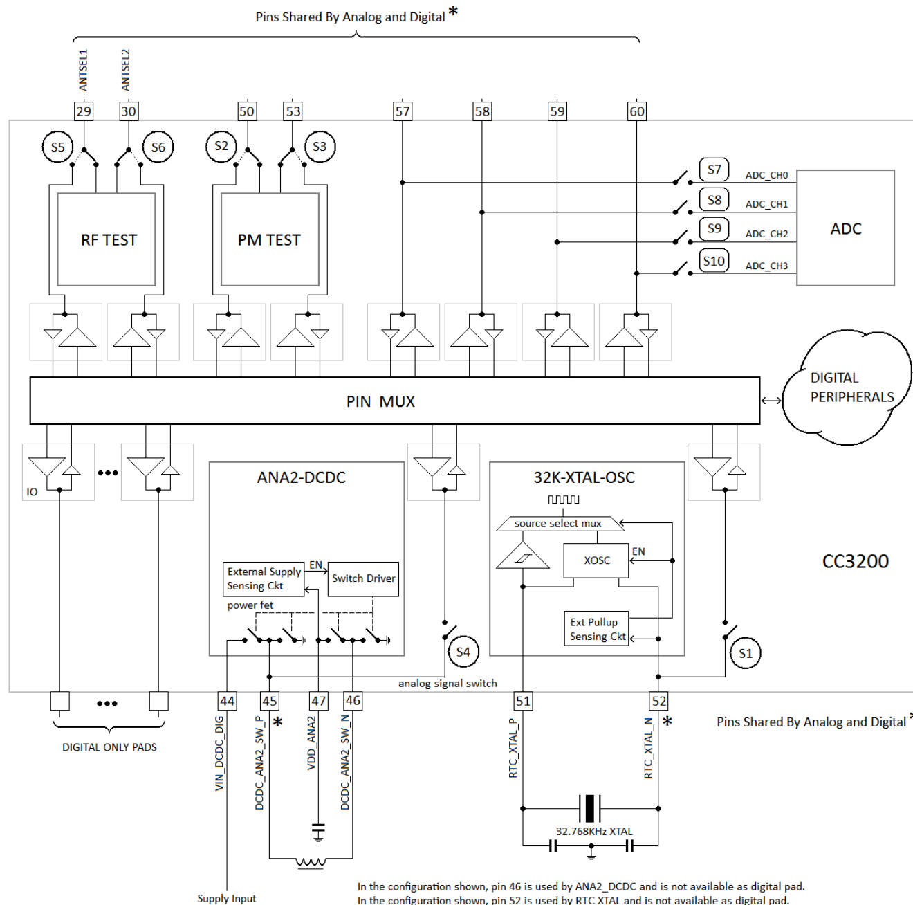
Figure 16-1. Board Configuration to Use Pins 45 and 52 as Digital Signals
