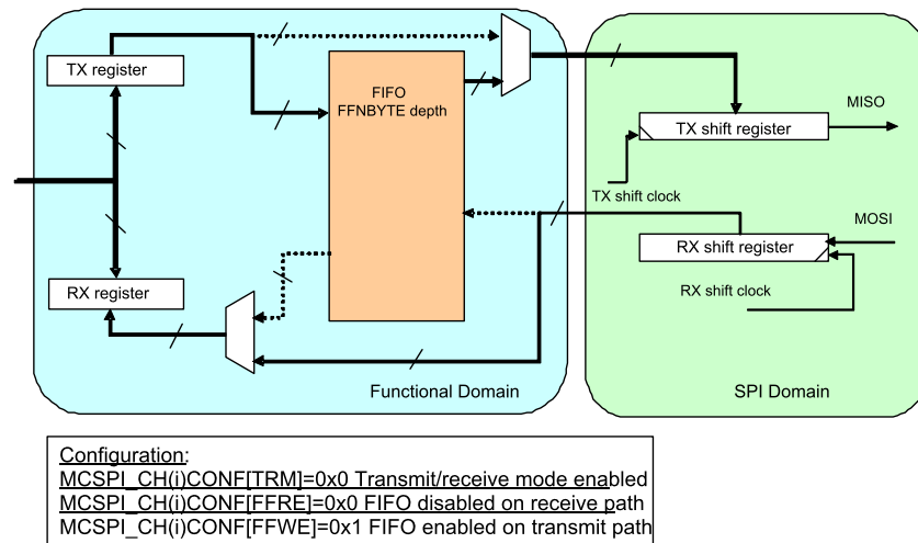
Figure 8-8. Transmit/Receive Mode With Only Transmit FIFO Used
