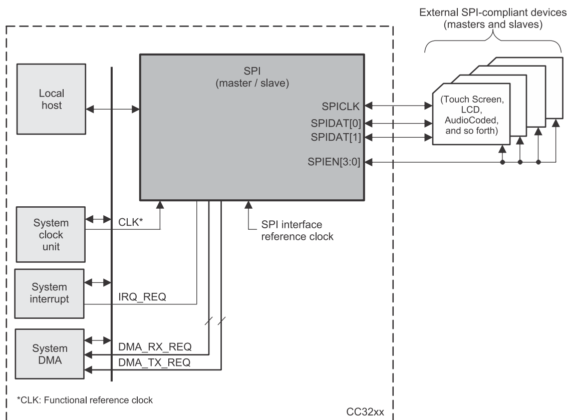
Figure 8-1. SPI Block Diagram
