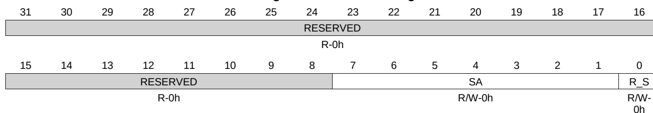
Figure 7-14. I2CMSA Register
