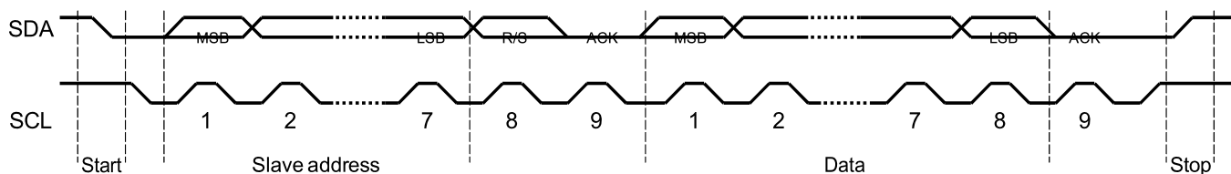
Figure 7-4. Complete Data Transfer with a 7-Bit Address
