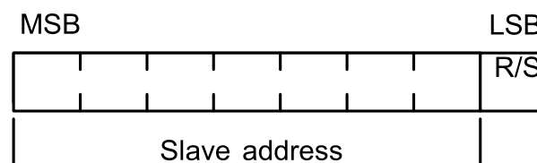
Figure 7-5. R/S Bit in First Byte
