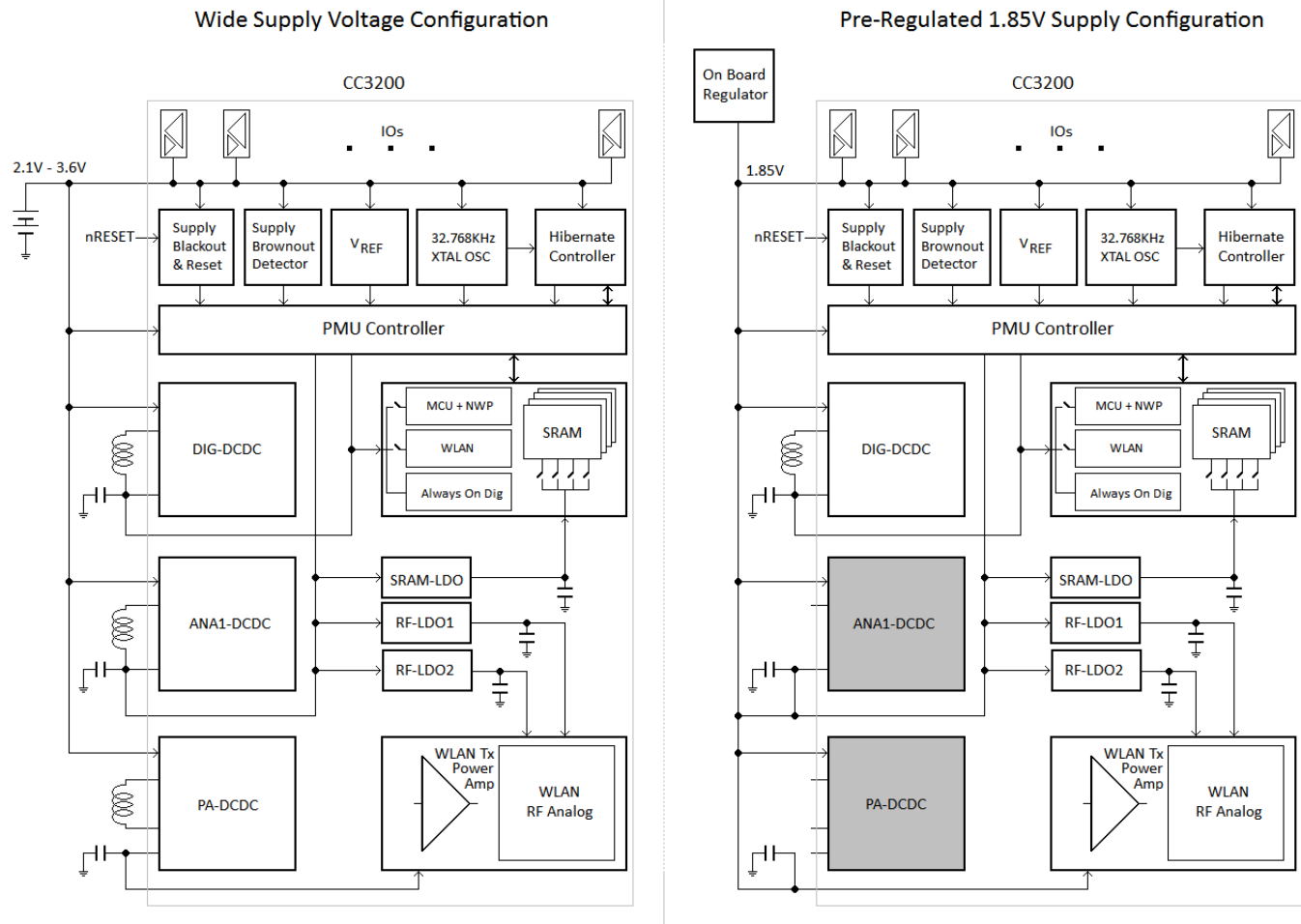
Figure 15-1. Power Management Unit Supports Two Supply Configurations
