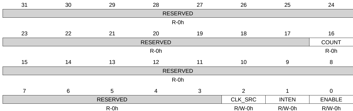
Figure 3-2. STCTRL Register
