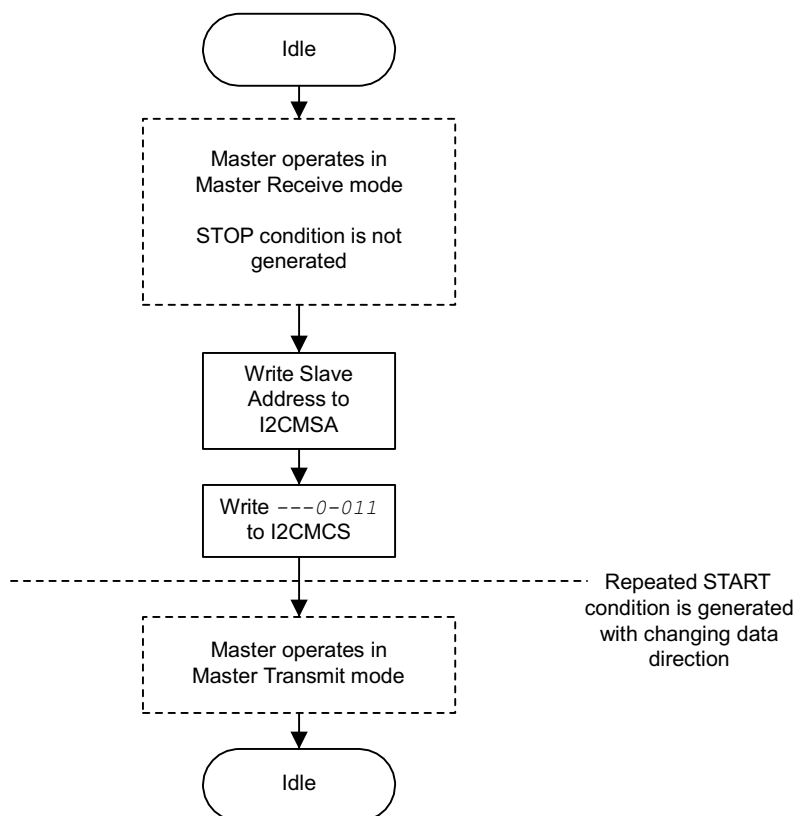
Figure 7-12. Master TRANSMIT with Repeated START after Master RECEIVE
