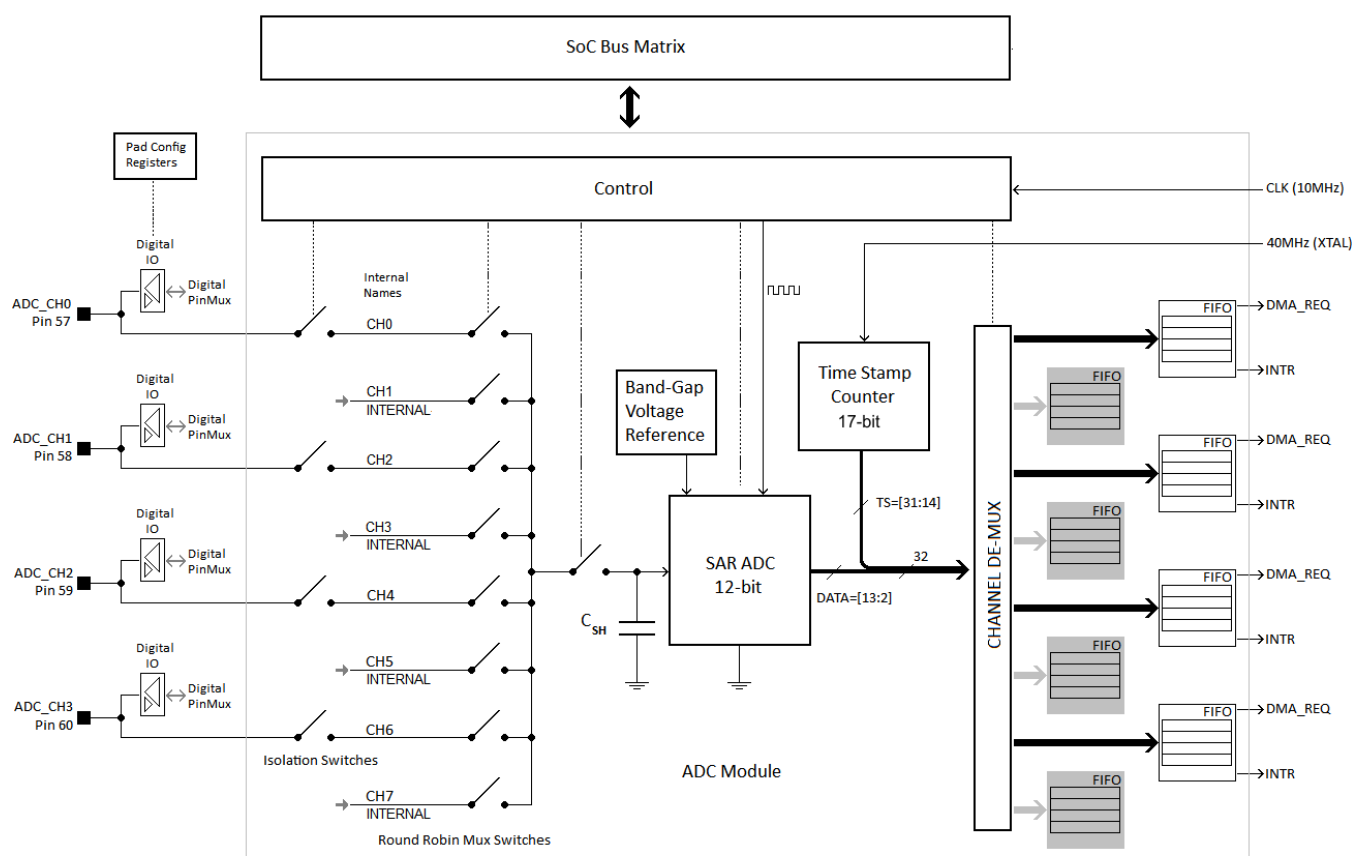
Figure 13-1. Architecture of the ADC Module in CC3200
