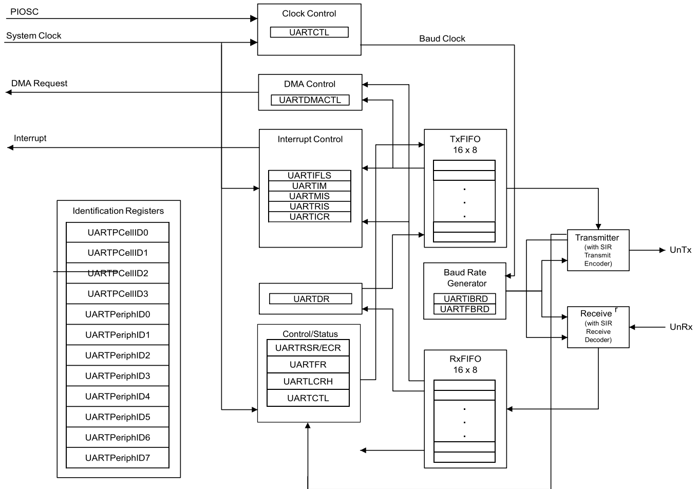
Figure 6-1. UART Module Block Diagram
