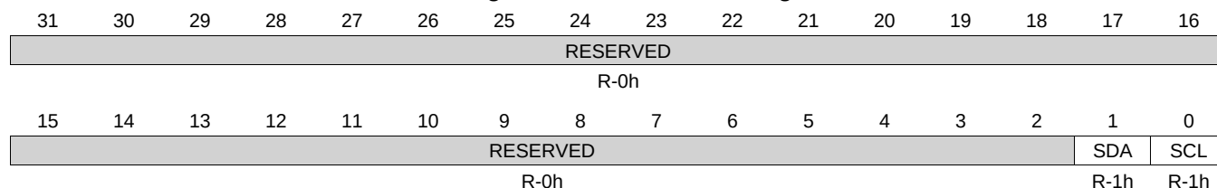
Figure 7-24. I2CMBMON Register
