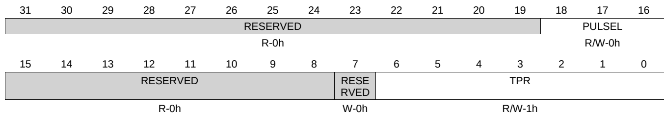
Figure 7-17. I2CMTPR Register
