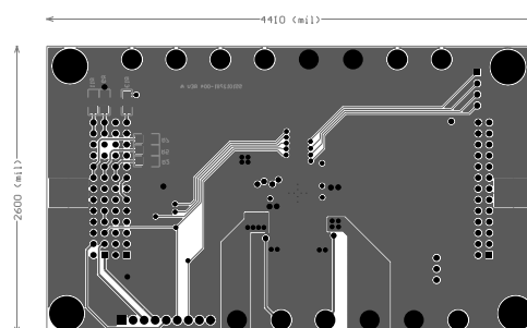
Figure 7. Bottom Layer
