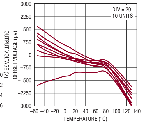
Output Offset Voltage vs Temperature
