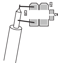
Figure 2. Measuring Output Ripple
