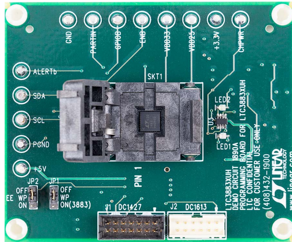
Figure 2. Open Shell. Verify IC Installed
