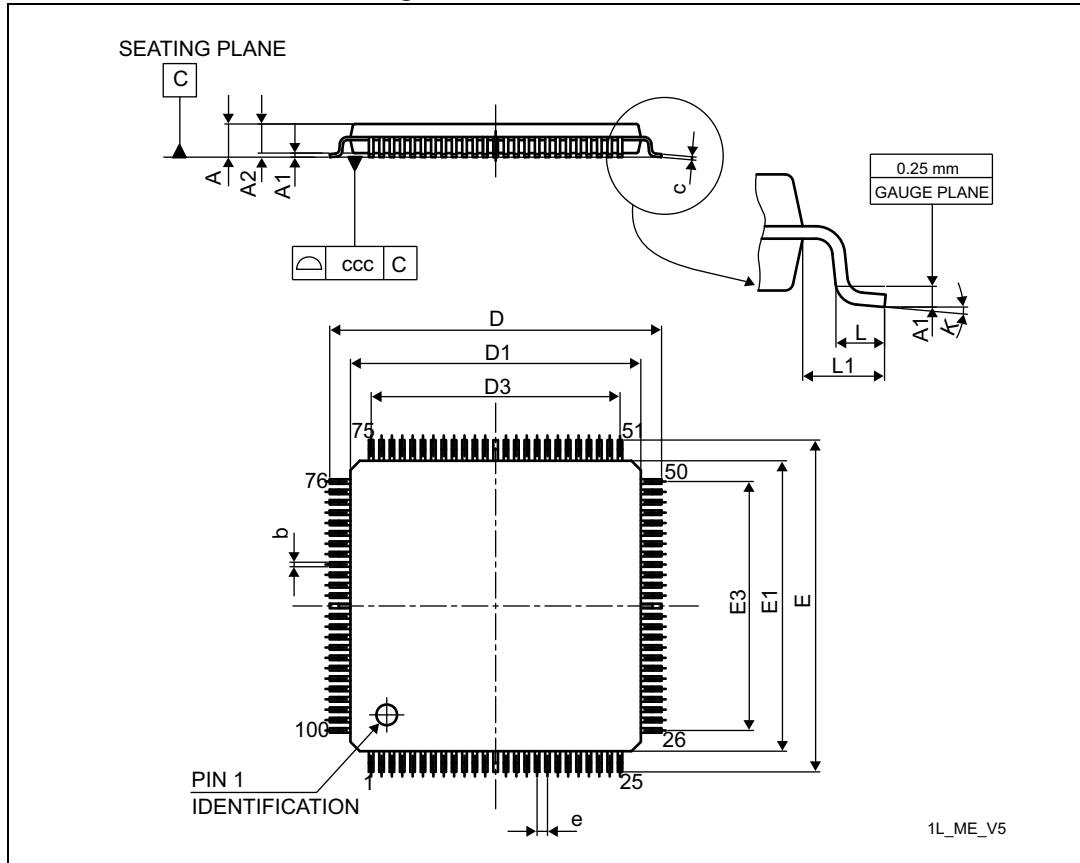
Figure 86. LQFP100 outline
