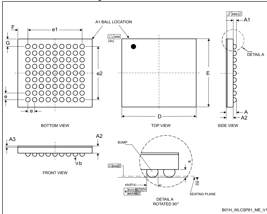
Figure 83. WLCSP81 outline
