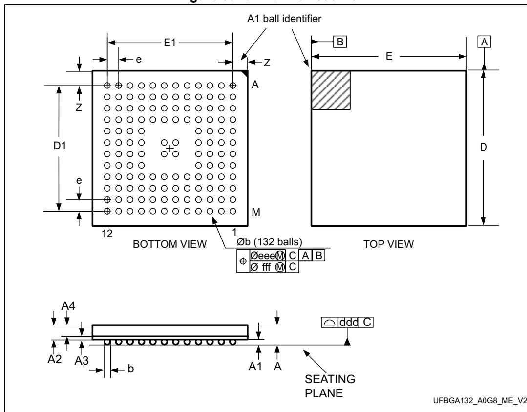
Figure 89. UFBGA132 outline
