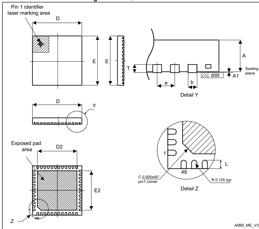
Figure 77. UFQFPN48 outline
