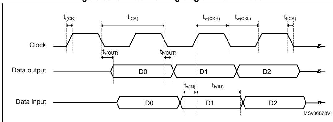
Figure 65. OCTOSPI timing diagram - SDR mode
