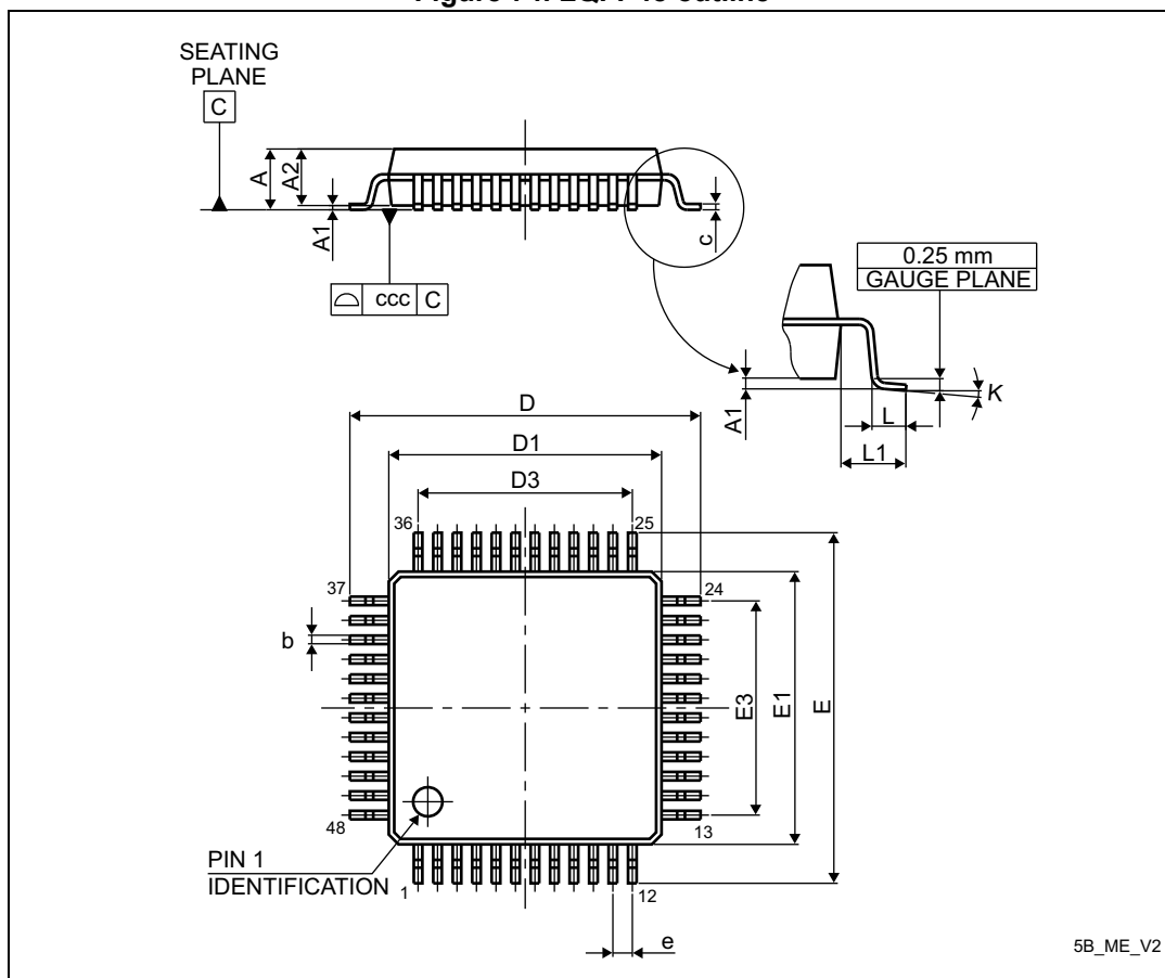
Figure 74. LQFP48 outline
