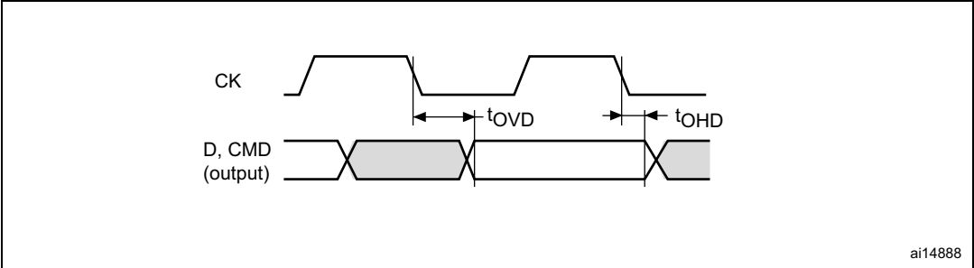
Figure 72. SD default mode
