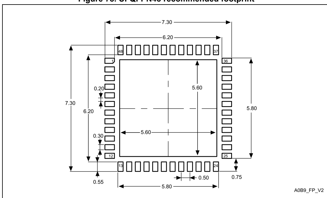
Figure 78. UFQFPN48 recommended footprint
