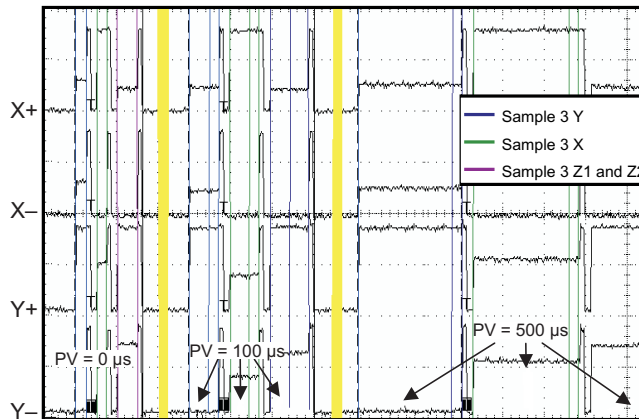
Figure 54. Panel Voltage Stabilization 0 \mu s, 100 \mu s, and 500 \mu s
