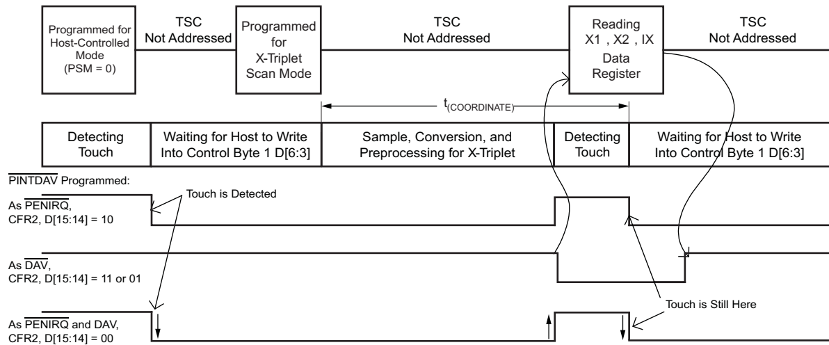
Figure 28. Example of a Single X-Triple Touch-Screen Scan (With Panel Stabilization Time) Using TSMODE 3
