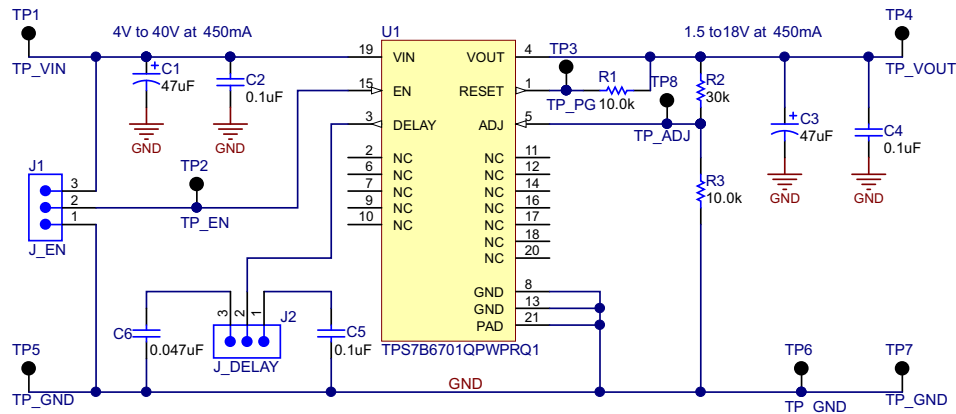
Figure 4. TPS7B6701EVM Schematic
