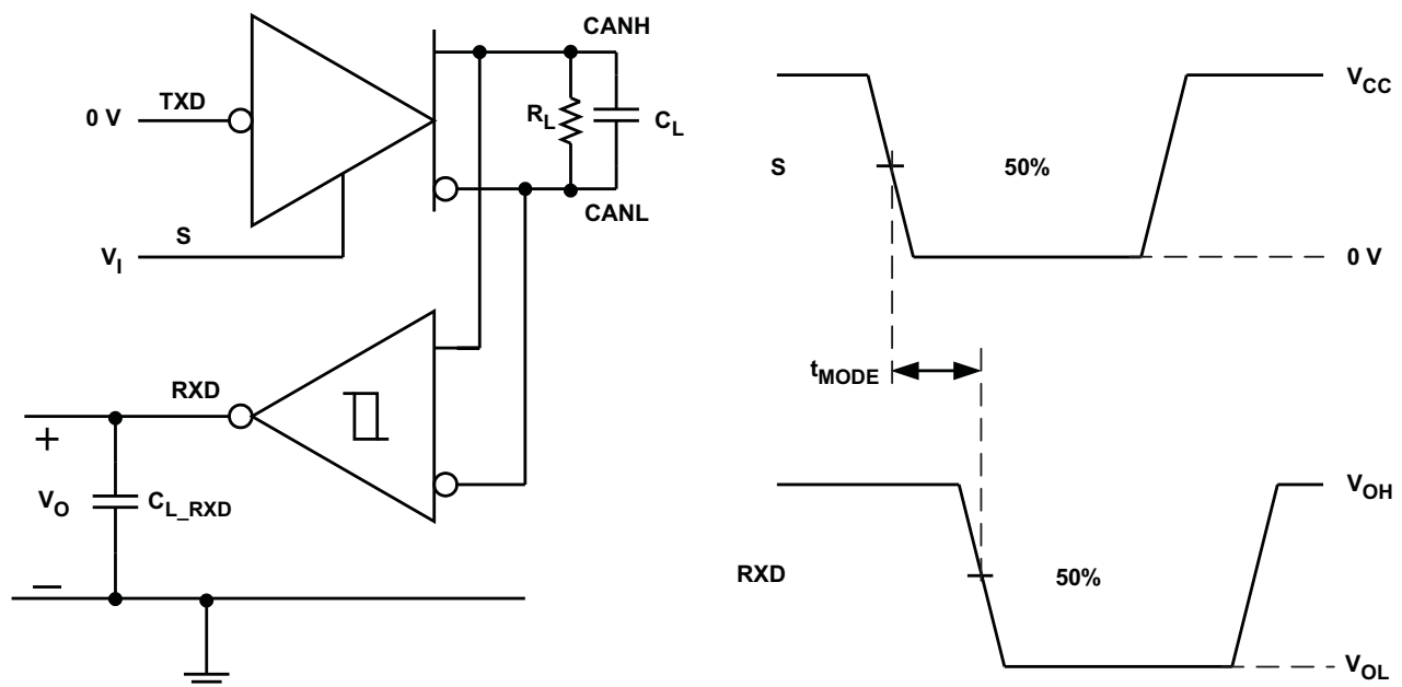
Figure 6. t_{\text{MODE}} Test Circuit and Measurement
