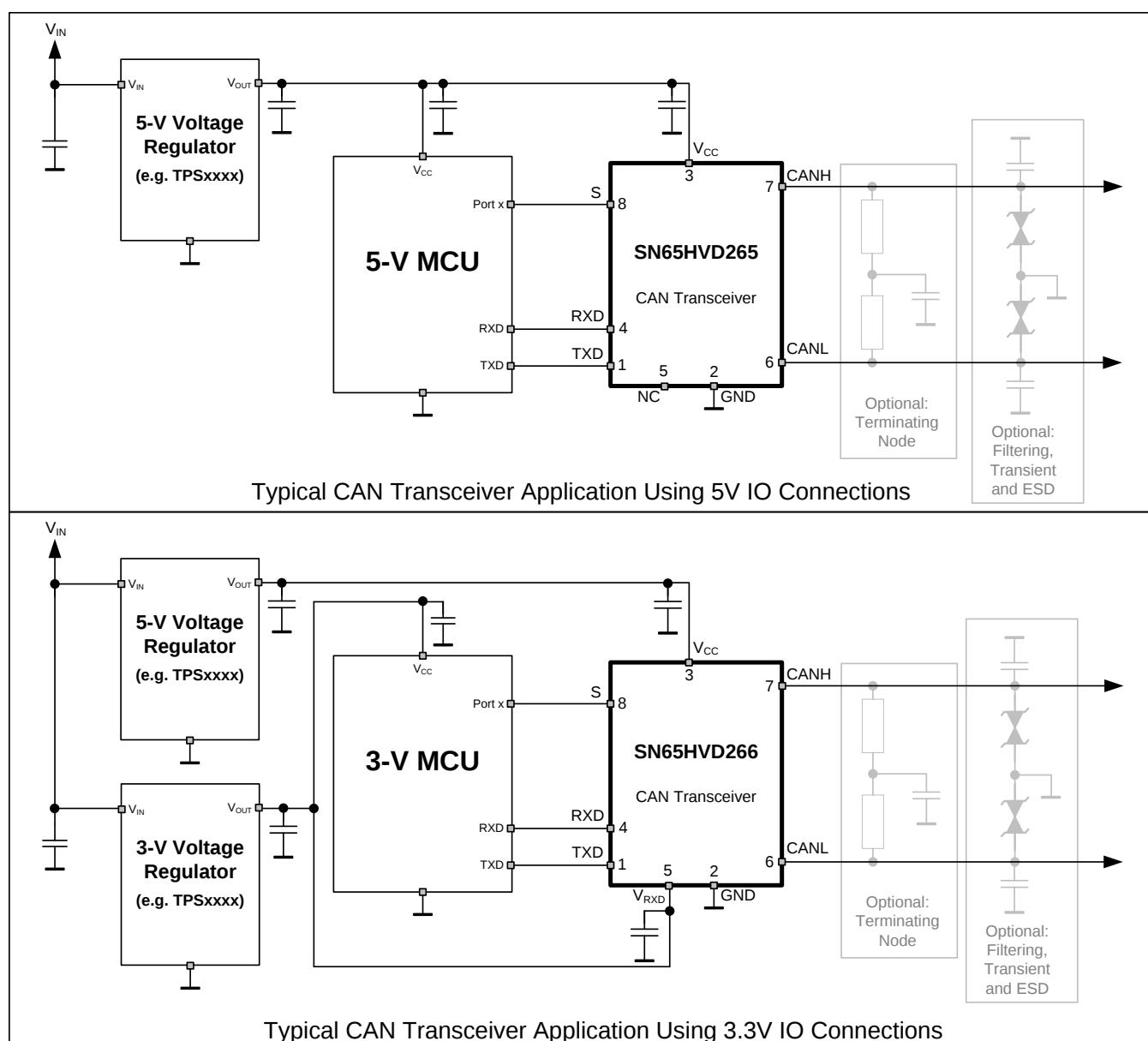
Figure 16. Typical 5-V Application
