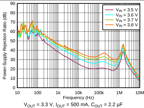
Figure 25. PSRR vs Frequency and V_{IN}
