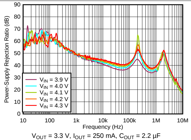
Figure 28. PSRR vs Frequency and V_{IN}
