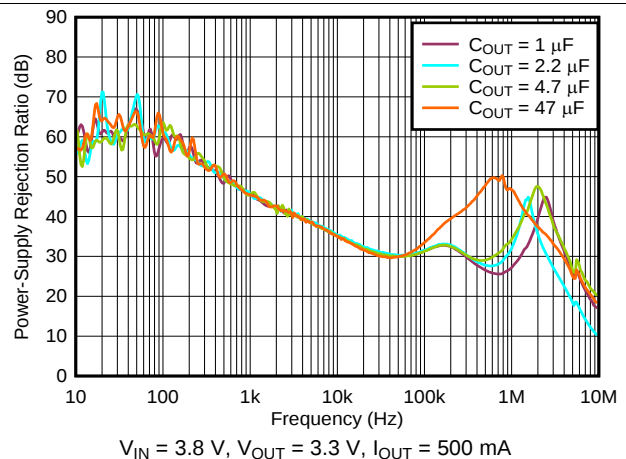
Figure 30. PSRR vs Frequency and C_{OUT}
