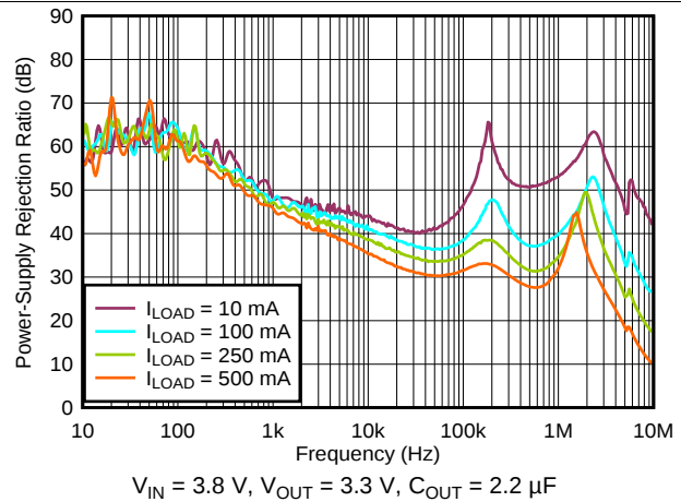
Figure 32. PSRR vs Frequency and I_{LOAD}
