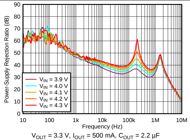
Figure 26. PSRR vs Frequency and V_{IN}
