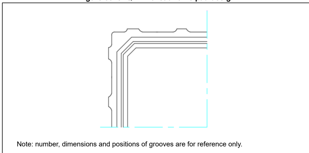
Figure 58. eLQFP176 leadframe pad design
