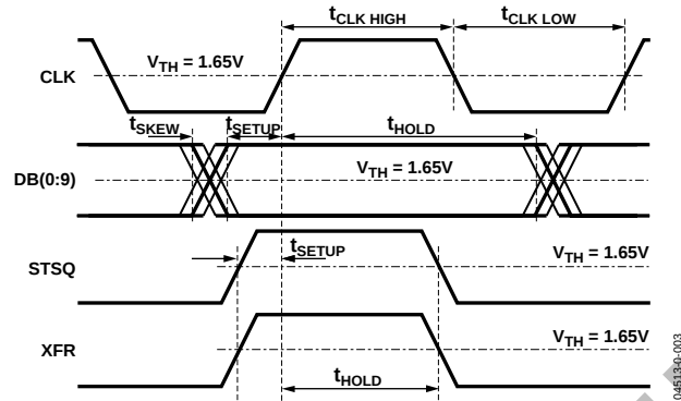
Figure 3. Timing Diagram, Even Mode ( E/O = \text{HIGH} )
