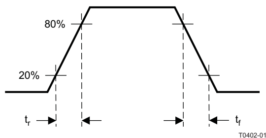
Figure 3. Output Rise and Fall Times
