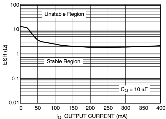
Figure 5. Output Stability with Output Capacitor ESR, Fixed Versions (5.0 V and 3.3 V)
