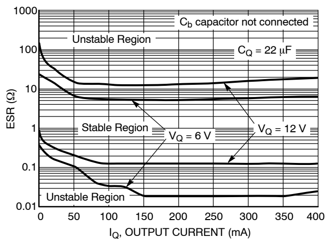
Figure 8. Output Stability with Output Capacitor ESR, Adjustable Version
