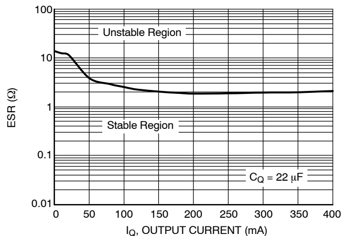
Figure 6. Output Stability with Output Capacitor ESR, Fixed Versions (5.0 V and 3.3 V)
