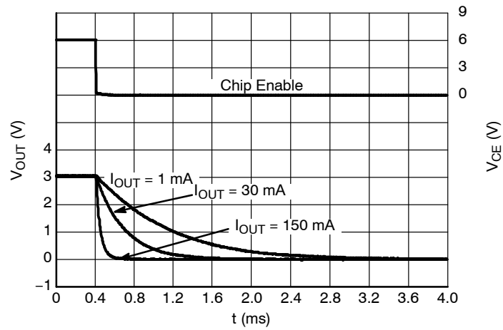
Figure 81. Shutdown, 3.0 V Version D, V_{IN} = 6.0 V
