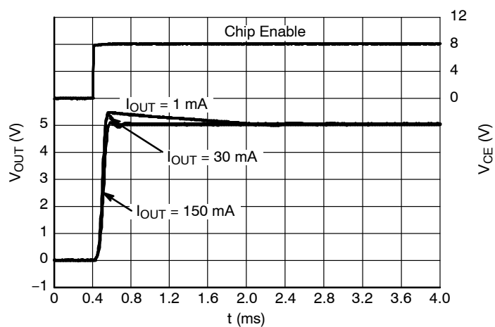
Figure 79. Start-up, 5.0 V Version, V_{IN} = 8.0 V, ECO = L
