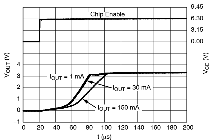
Figure 78. Start-up, 3.3 V Version, V_{IN} = 6.3 V, ECO = H
