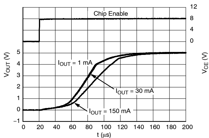
Figure 80. Start-up, 5.0 V Version, V_{IN} = 8.0 V, ECO = H
