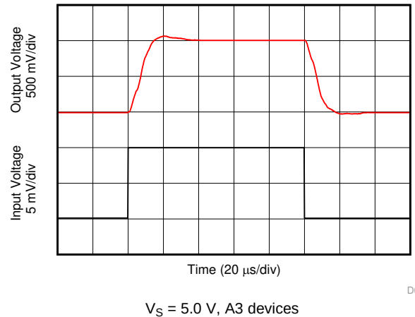
Figure 22. Step Response (10-mV PP Input Step)
