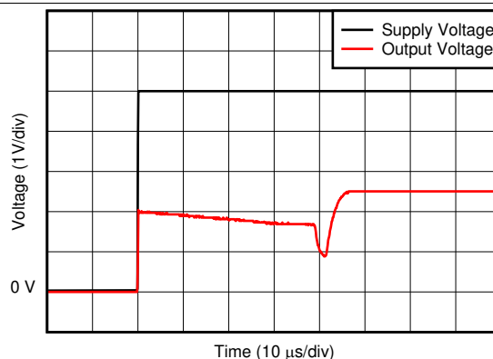
Figure 26. Start-Up Response
