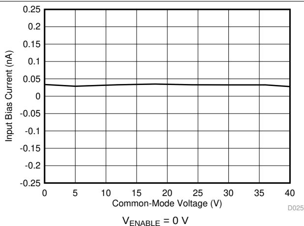
Figure 15. Input Bias Current vs Common-Mode Voltage (Shutdown)
