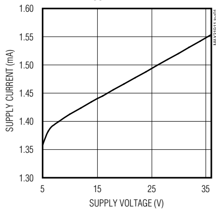
POWER-SUPPLY CURRENT vs. V_{\text{CC24V}} FIELD SUPPLY
