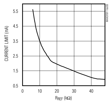
CURRENT LIMIT vs. R_{\text{REF}}
