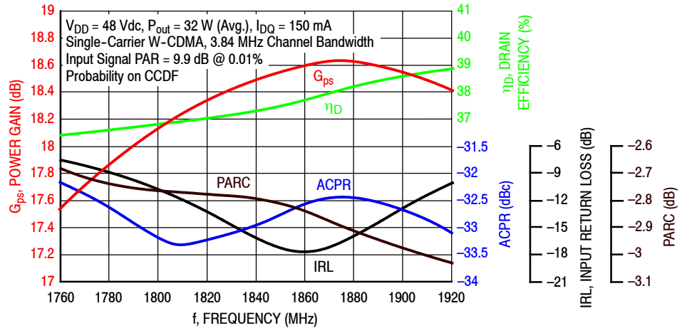
Figure 17. Single-Carrier Output Peak-to-Average Ratio Compression (PARC) Broadband Performance @ P_{out} = 32 \text{ Watts Avg.}
