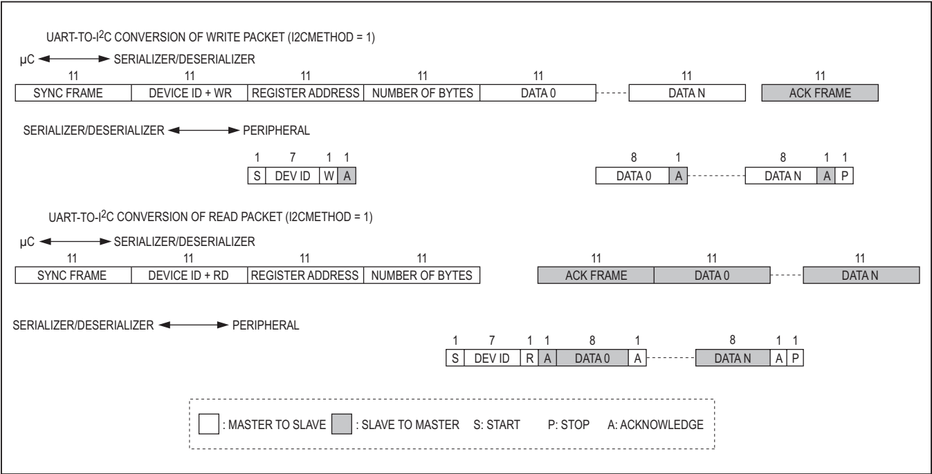
Figure 32. Format Conversion Between GMSL UART and I2C without Register Address (I2CMETHOD = 1)
