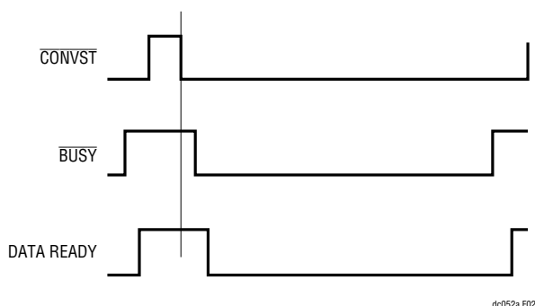
Figure 2. Timing Diagram
