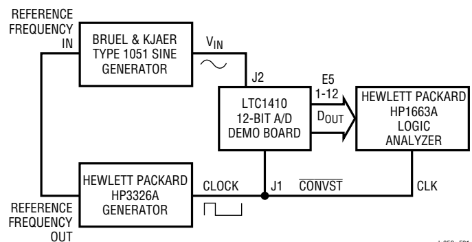
Figure 1. Typical Setup for LTC1410 Demo Board
