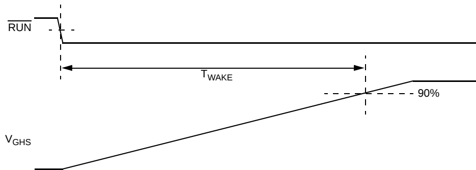
Figure 5. High-Side Gate-Drive Supply Wake-Up Time “Twake”
