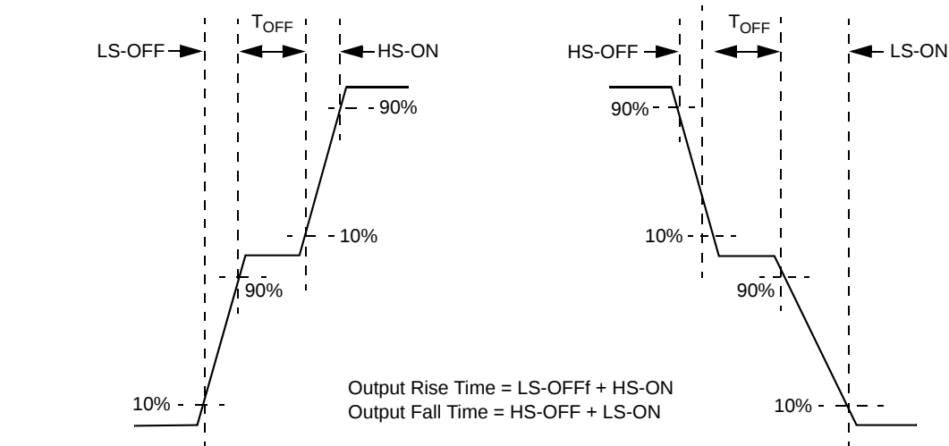
Figure 8. Rise Time, Fall Time, Shoot Through Prevention Timing
