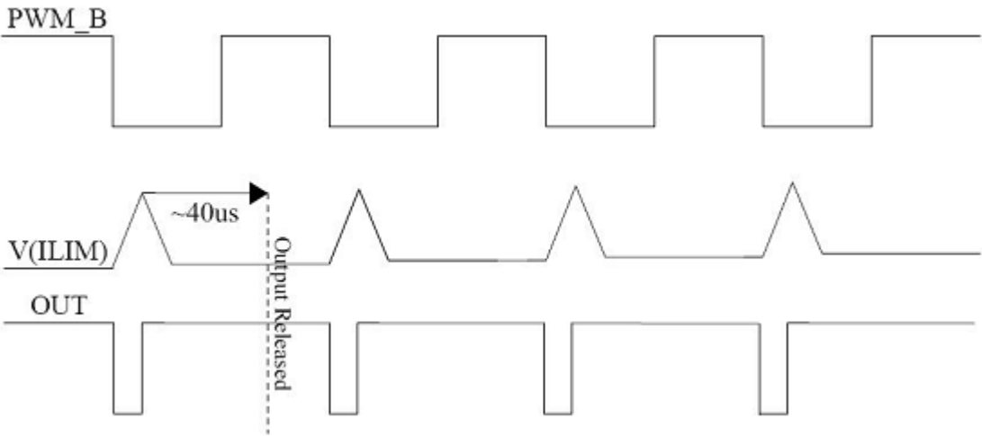
Figure 13. ISEN Current Limit Waveforms
