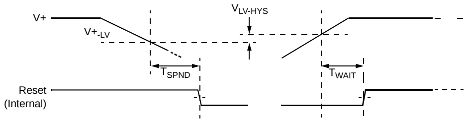
Figure 6. Timing for Reset on Low V+ Detect
