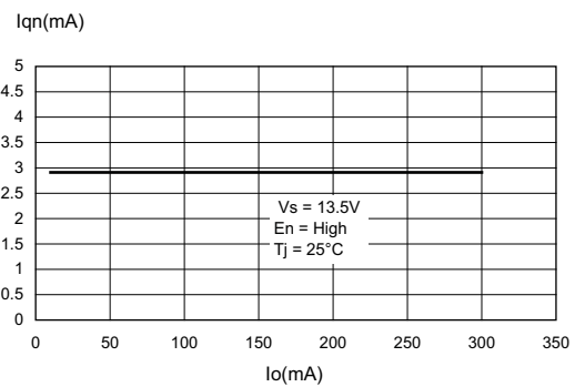
Figure 6. Current consumption vs output current
