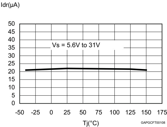
Figure 17. I_{dr} vs T_j
