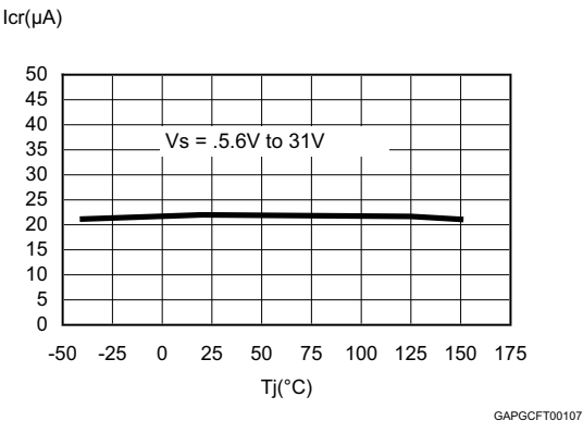
Figure 16. I_{cr} vs T_j
