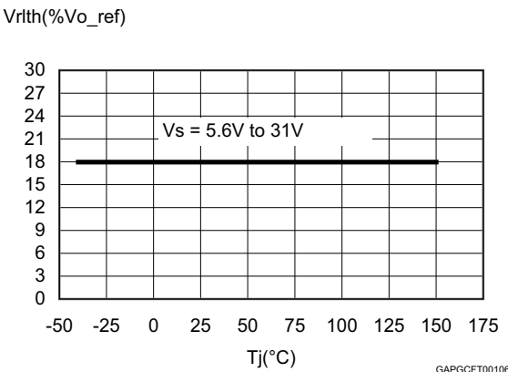
Figure 15. V_{Rlth} vs T_j
