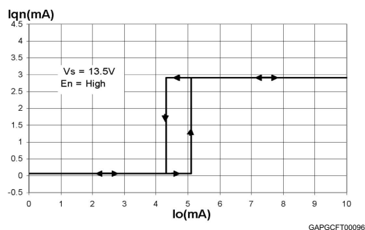
Figure 7. Current consumption vs output current (at light load condition)
