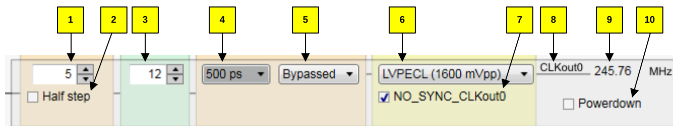
Figure 2. Clock Outputs Page CLKout Path Description Diagram
