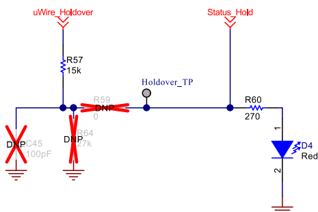
Figure 9. Digital
