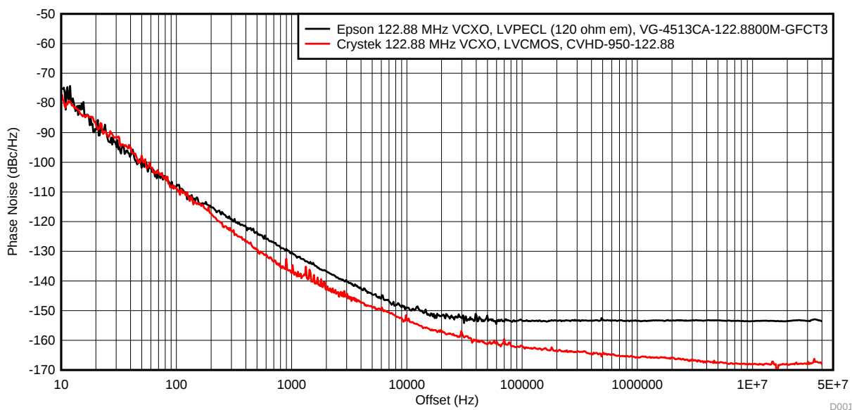
Figure 18. VCXO Phase Noise at 122.88 MHz
