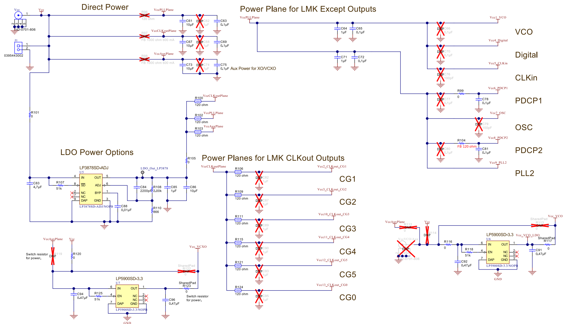
Figure 7. Power Supply
