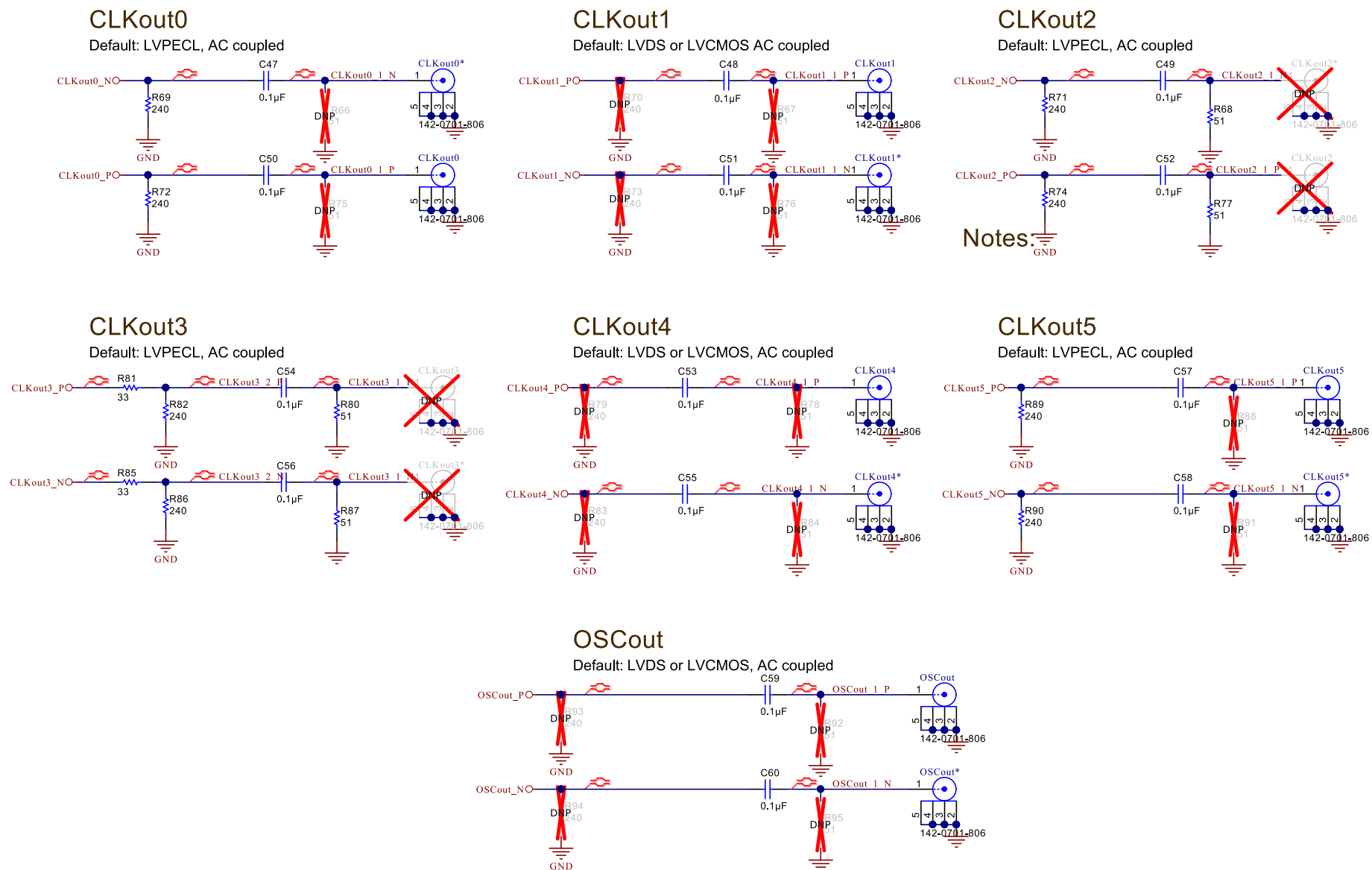
Figure 11. Clock Outputs
