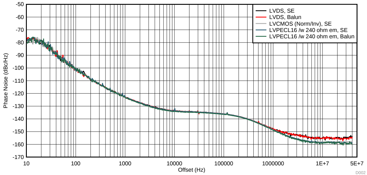
Figure 19. LMK04208 245.76 MHz, Divide-by-12
