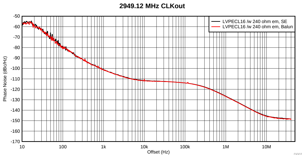
Figure 20. LMK04208, 2949.12 MHz, Divide-by-1
