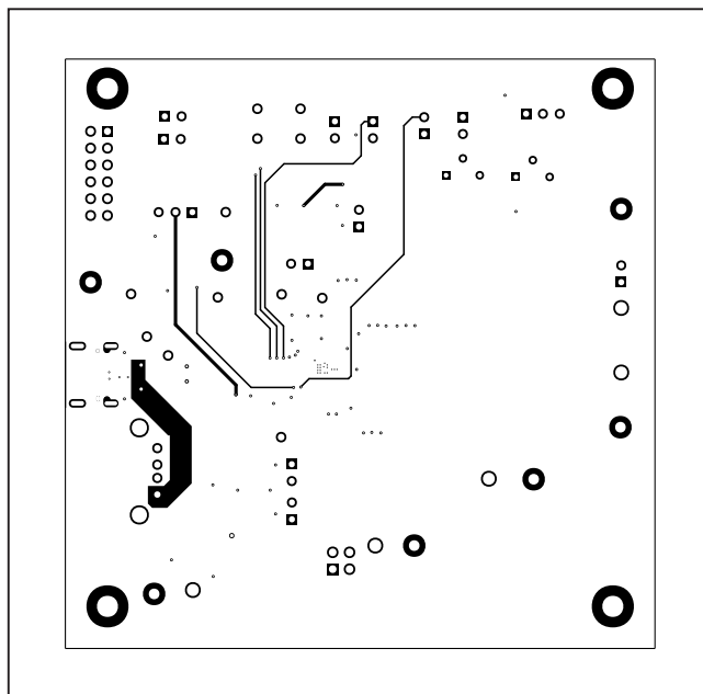
MAX14748 EV Kit—Level 3 SIGS
