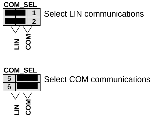
Figure 8: COM_SEL Option Header
