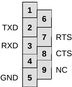
Figure 9: COM Connector
