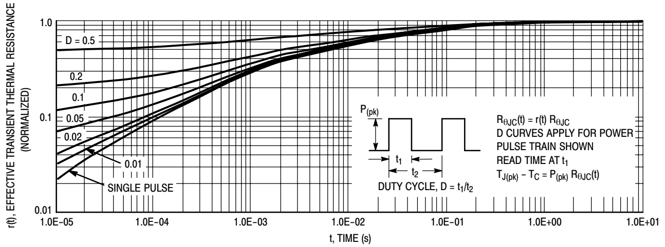
Figure 14. Thermal Response
