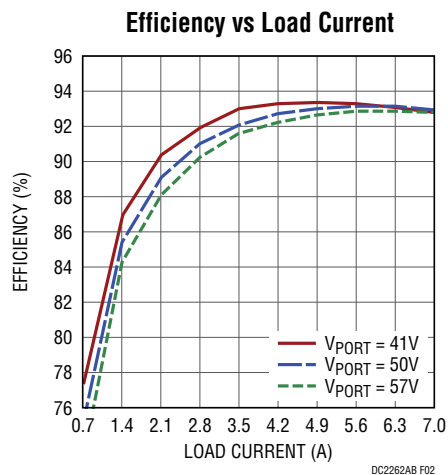
Figure 2. Efficiency (Ethernet Port to Output)
