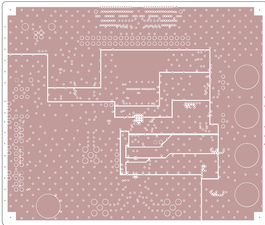
Figure 5. Power Plane
