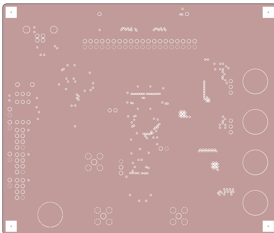
Figure 4. Ground Plane
