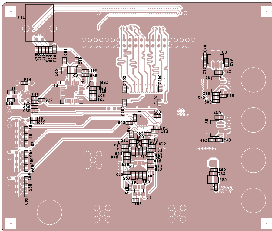
Figure 6. Bottom Silkscreen
