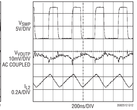
Switching Waveform at 100mA Load (Boost)
