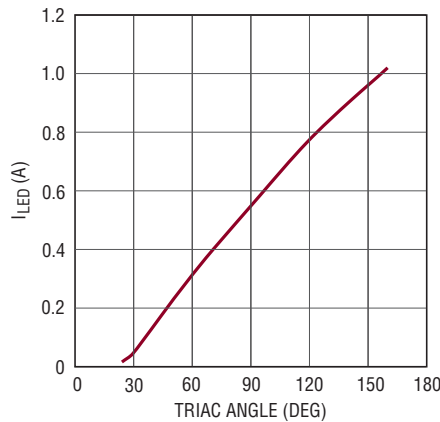
Figure 2. LED Current vs TRIAC Angle (120V AC Application)
