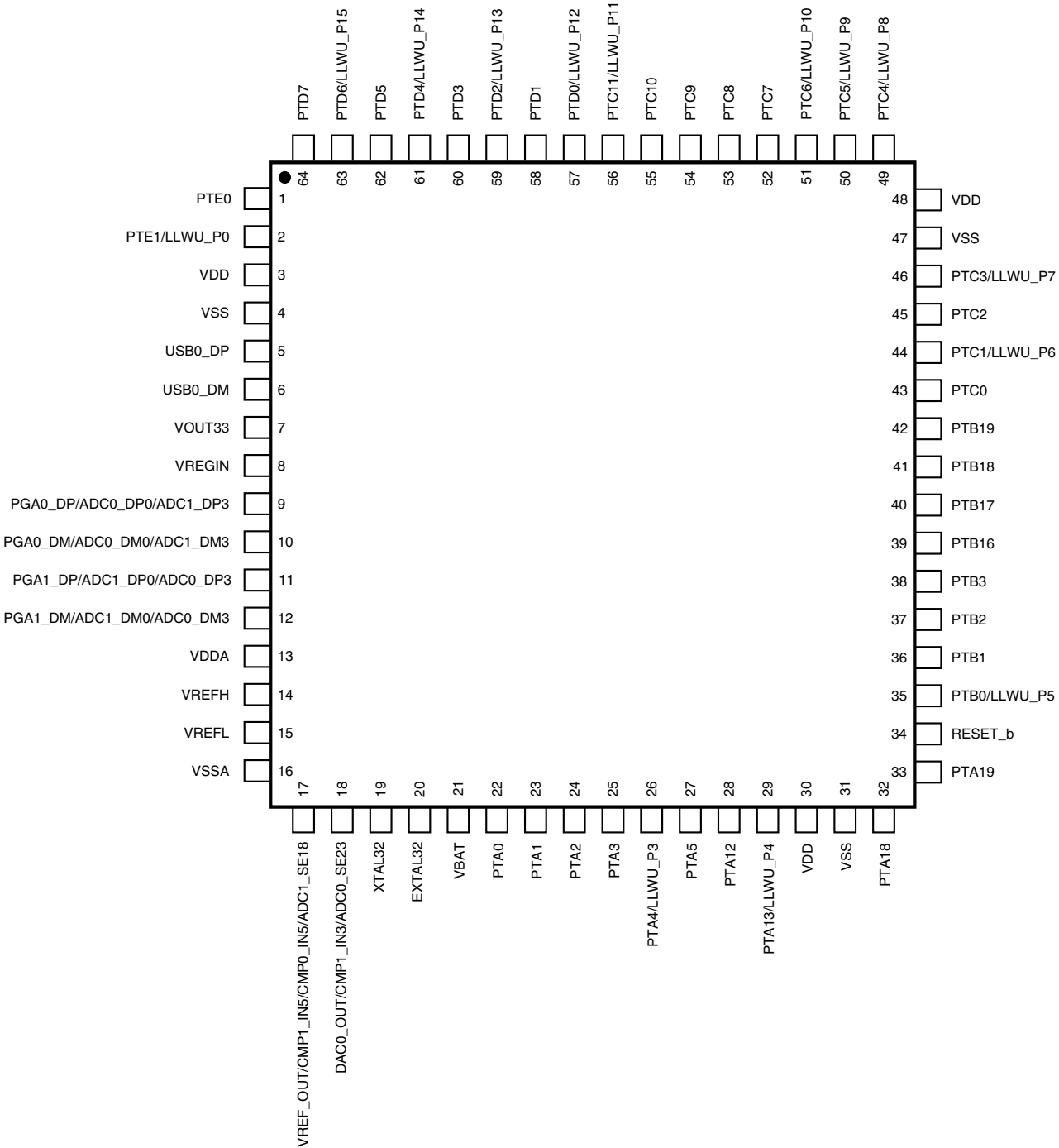
Figure 10-2. K20 64 LQFP/QFN Pinout Diagram
