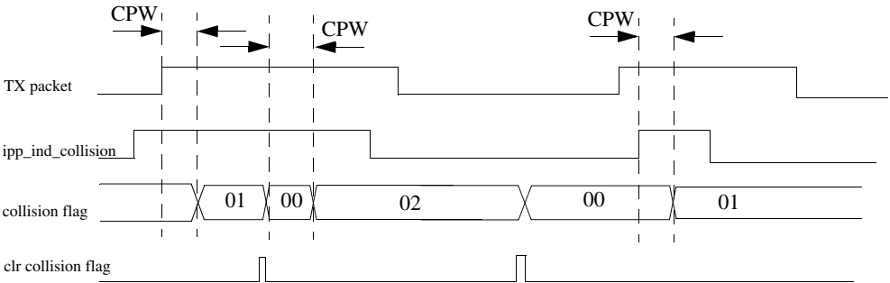
Figure 47-53. Collision pulse detection
