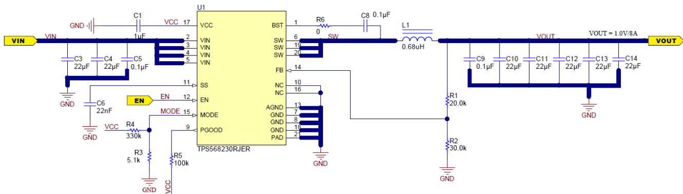
Figure 30. 1-V, 8-A Reference Design with Eco-mode, F_{SW} = 600 \text{ kHz}
