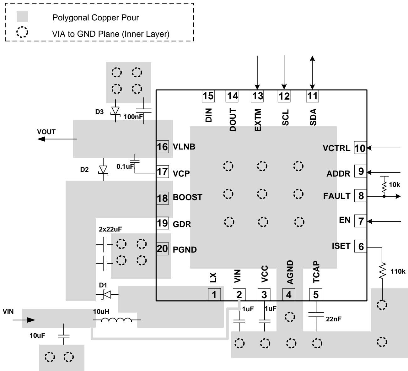
Figure 40. Layout
