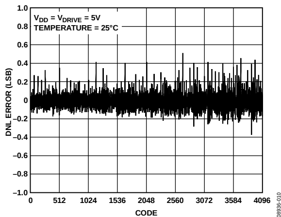
Figure 7. Typical DNL
