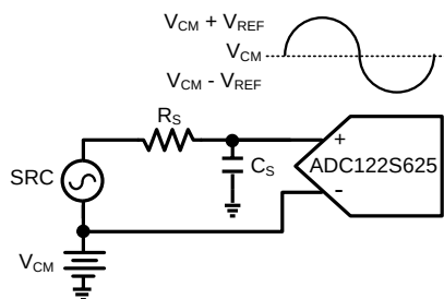
Figure 35. Single-Ended Input
