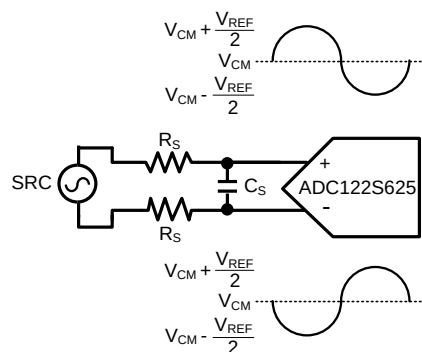
Figure 34. Differential Input
