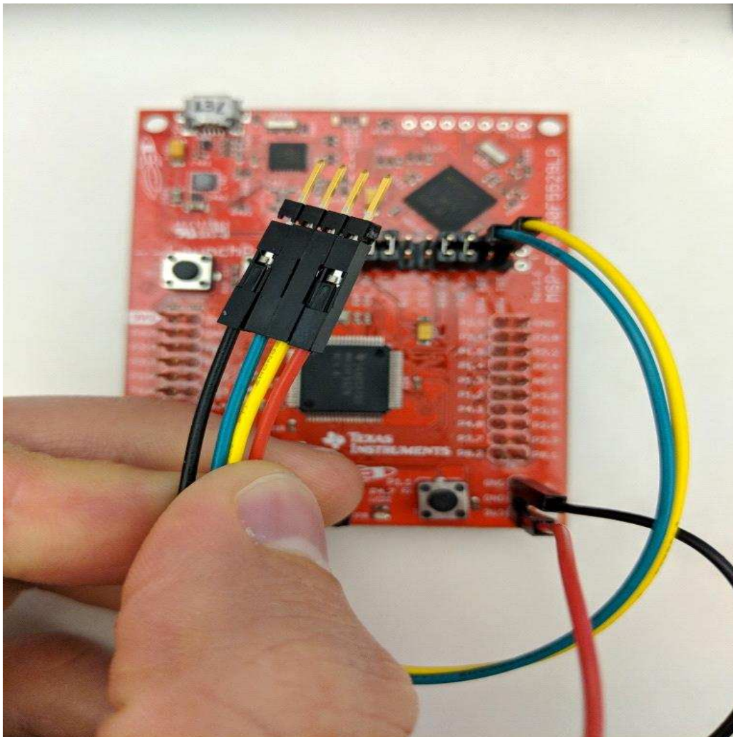
Figure 17. Wiring Connection
