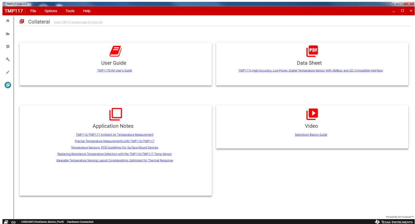
Figure 25. Collateral Tab
