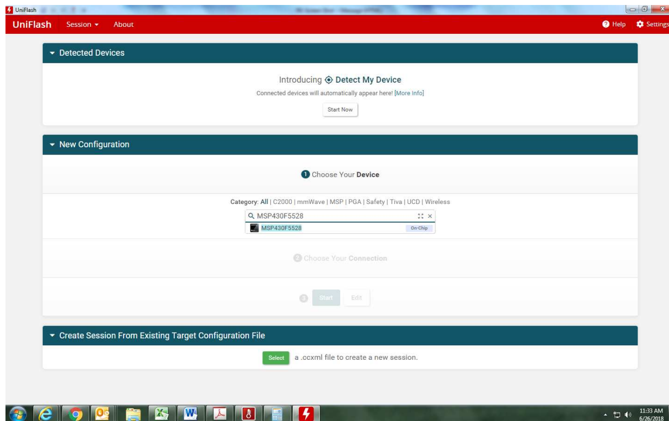
Figure 18. UniFlash GUI
