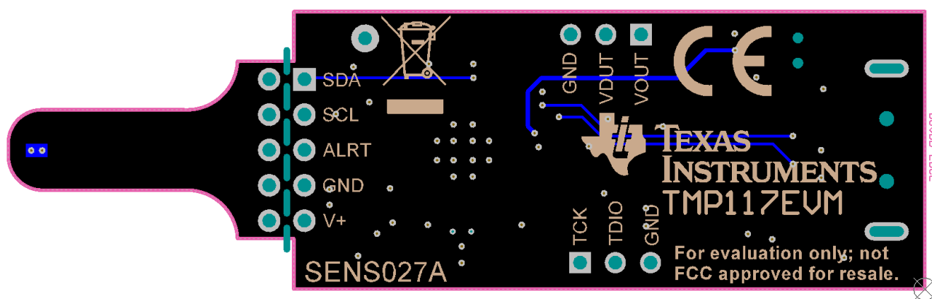
Figure 31. Bottom Assembly Layer
