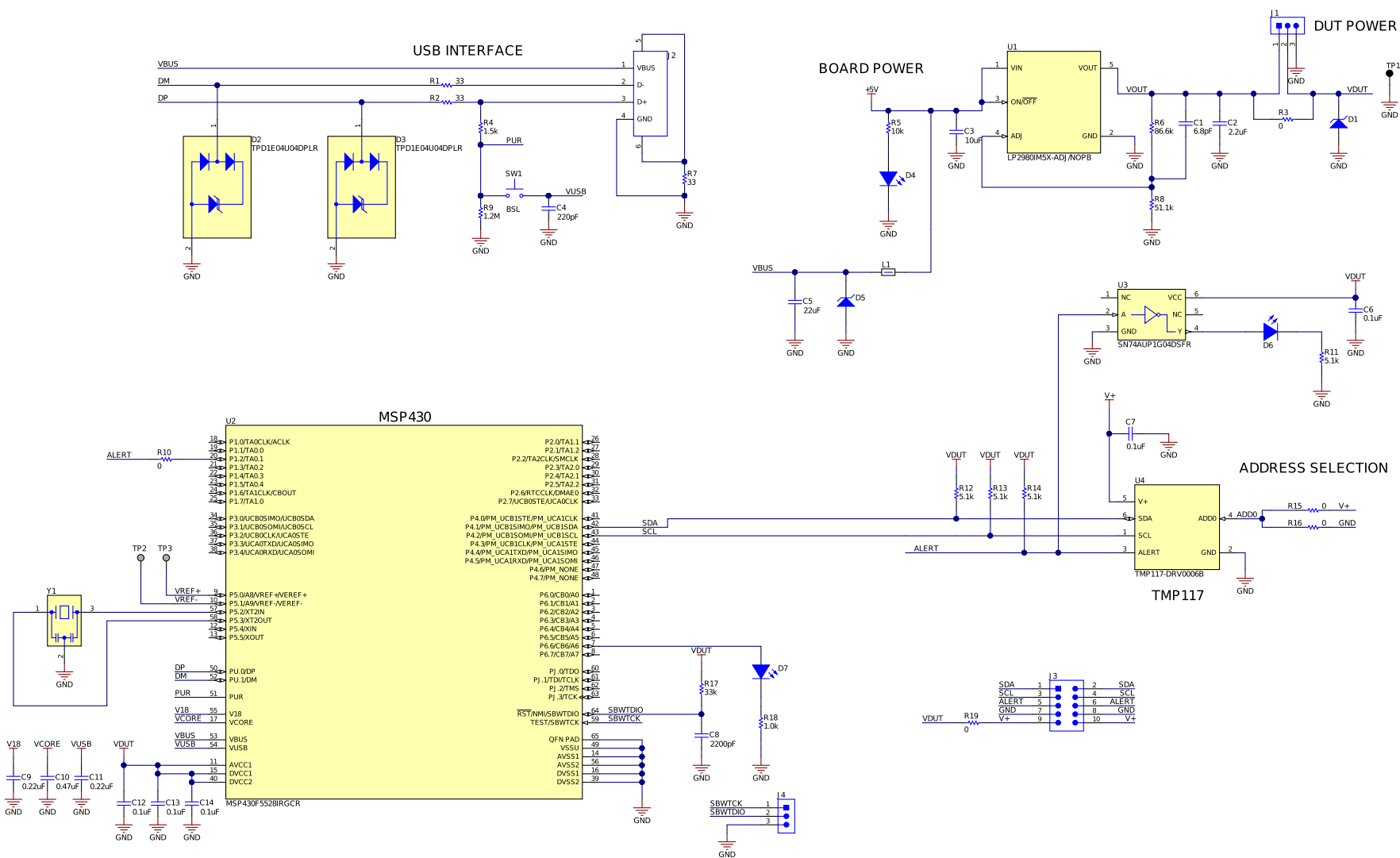
Figure 32. TMP117EVM Schematic
