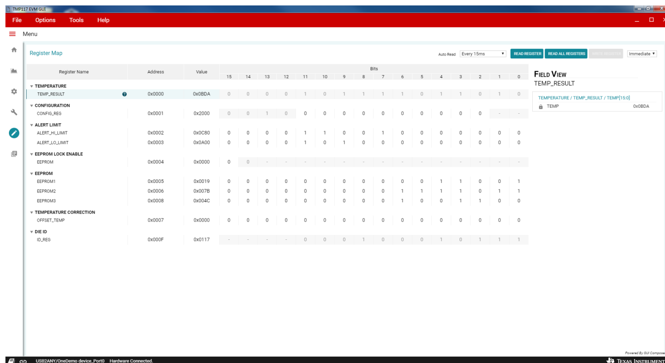
Figure 24. Registers Tab
