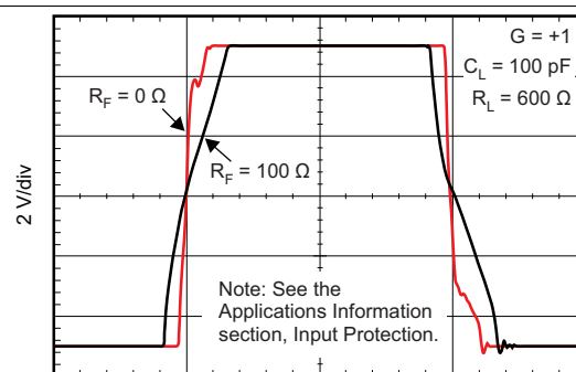
Time (0.5 \mu\text{s}/\text{div} )
