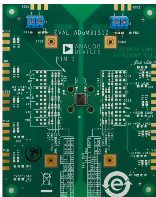
Figure 1. EVAL-ADuM3151Z Evaluation Board
