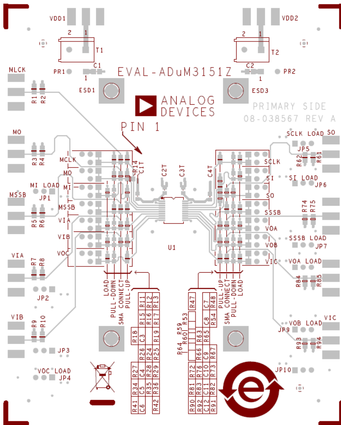
Figure 5. Top Side Layout
