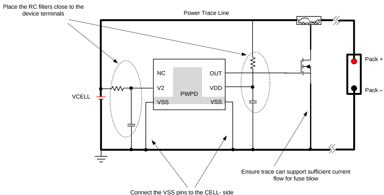
Figure 14. Layout Schematic
